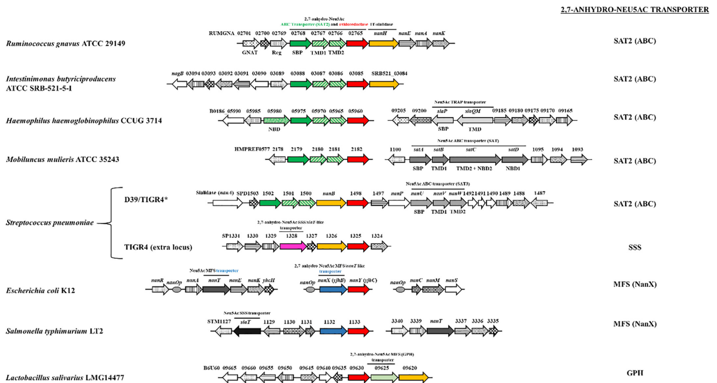
Figure 8. Diversity of 2,7-anhydro-Neu5Ac catabolic clusters among sialic acid-utilizing bacteria. Gene functions were inferred from BLAST searches followed by gene linkage and cluster analysis. Orthologous genes are identified with individual patterns. The genes encoding 2,7-anhydro-Neu5Ac transporters, 2,7-anhydro-Neu5Ac oxidoreductases, and IT-sialidases are distinguished by color for emphasis. Nomenclature is as follows: nanA , Neu5Ac lyase; nanK , N -acetylmannosamine kinase; nanE , N -acetylmannosamine-6-phosphate epimerase; nanC , Neu5Ac outer membrane channel; nanM , Neu5Ac mutarotase; nanS , N -acetyl-9- O -acetylneuraminic ester; nagB , glucosamine-6-phosphate deaminase; GNAT , GCN5-related N -acetyltransferase; Reg , regulator (please note that GNAT family proteins and regulator proteins, while recurrent within clusters, may belong to different clades and thus function differently in each organism); SAT2 , 2,7-anhydro-Neu5Ac transporter of the ABC superfamily; siaPQM , Neu5Ac transporter of the TRAP family; satABCD , Neu5Ac transporter of the ABC superfamily (SAT); nanUVW (SAT3), Neu5Ac transporter of the ABC superfamily (also named satABC ); nanT , Neu5Ac transporter of the MFS superfamily; siaT , Neu5Ac transporter of the SSS family; nanX ( yjhB ), 2,7-anhydro-Neu5Ac transporter ( nanT -like) of the MFS superfamily ABC; MFS , major facilitator superfamily; SSS , sodium solute symporter family; GPH , glycoside-pentoside-hexuronide:cation symporter family; SBP , solute-binding protein; TMD , transmembrane domain; NBD , nucleotide-binding domain. Note that the classification of ABC sialic acid transporters follows Almagro-Moreno and Boyd (34). *, TIGR4 possesses both the conserved sialic acid “supercluster,” as in strain D39, and an additional, candidate 2,7-anhydro-Neu5Ac cluster bearing the siaT -like transporter gene. In TIGR4, the conserved supercluster bears a minor difference in the form of pseudogenes and insertions (66).
