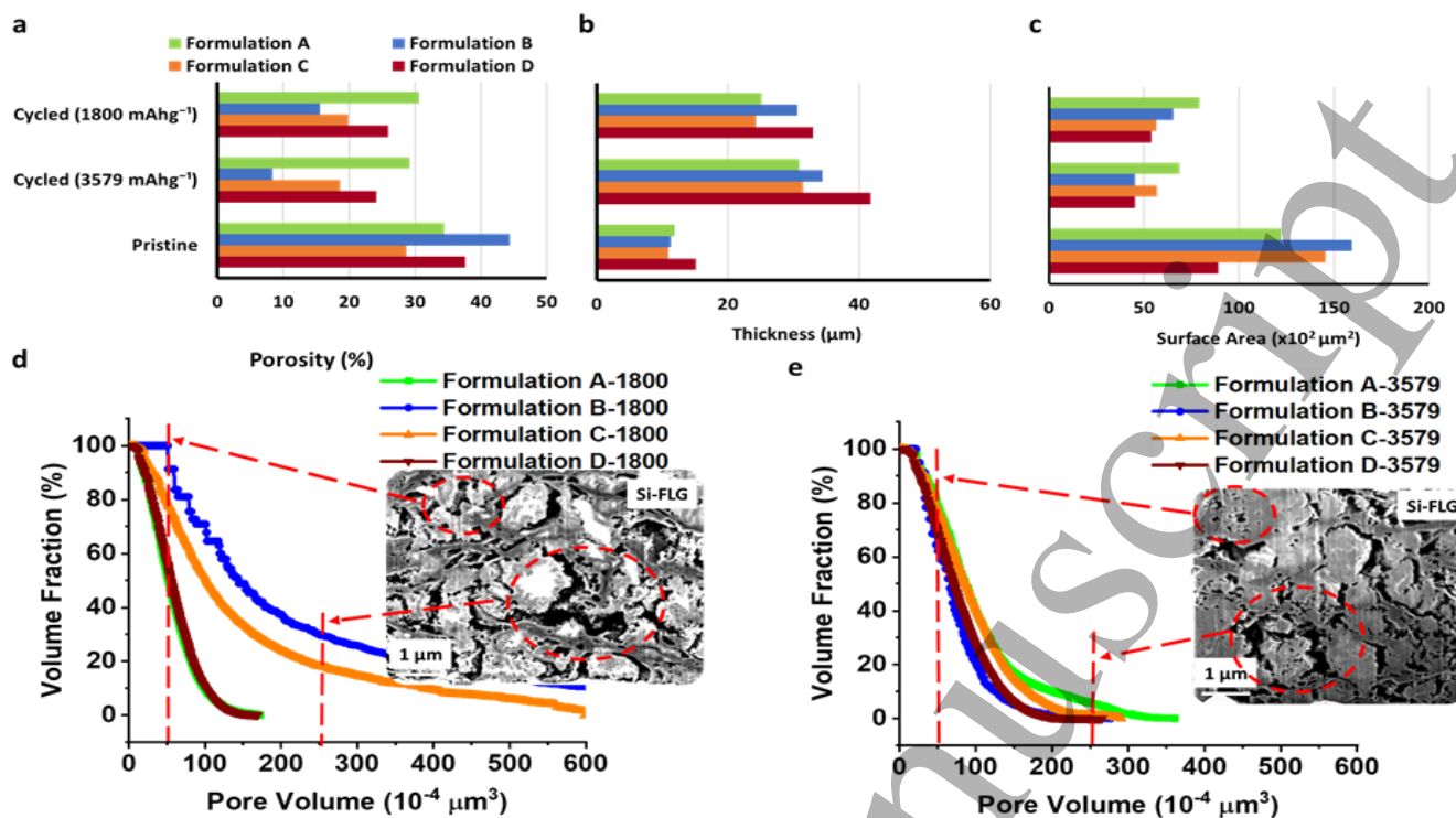
Figure 5. Geometrical property comparison after cycling at silicon's half and full capacity. Electrode's (a) porosity, (b) thickness and (c) pore surface area comparison; cumulative pore volume distribution comparison of all cycled electrodes with (d) half capacity of silicon, (e) full capacity of silicon (the insets show cross-sectional SEM images for Formulation A after 200 cycles under half and full capacity, respectively). The legends for (a) also applies to (b,c).
