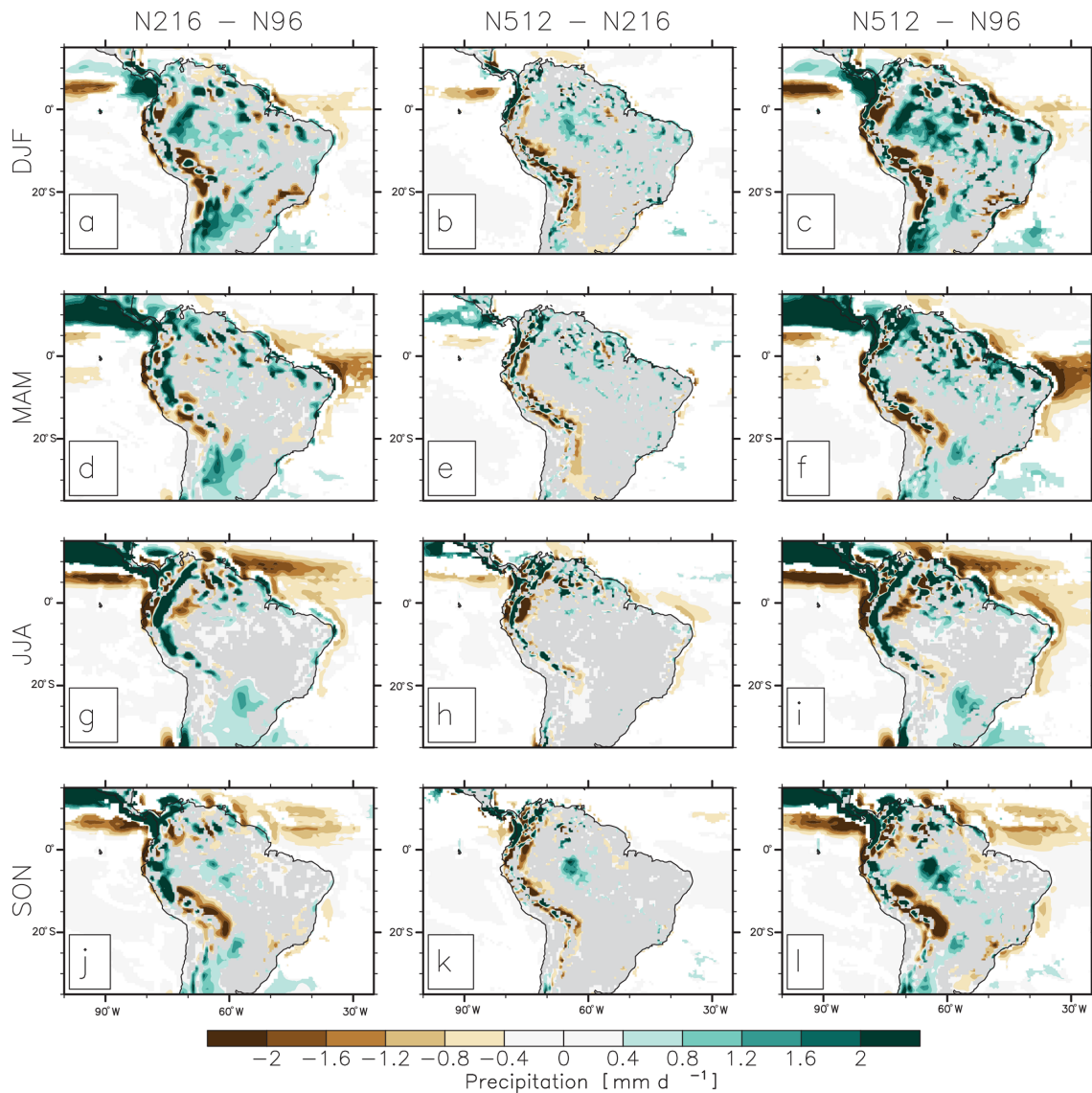
Figure 3. Ensemble-mean N216–N96 difference in (a) DJF, (d) MAM, (g) JJA, and (j) SON precipitation ( \text{mm d}^{-1} ). (b, e, h, k) As in (a), (d), (g), and (j) but for N512–N216. (c, f, i, l) As in (a), (d), (g), and (j) but for N512–N96. Differences are shown when statistically different to zero according to a Student’s t test and a 95 % confidence level.
