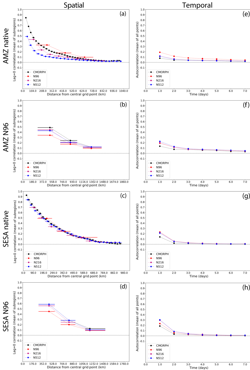
Figure 13. (a) Metric of the spatial scale of daily precipitation (at native resolution), computed by dividing the analysis domain into 1500 km × 1500 km subregions and calculating the mean lag-0 correlation between the central grid point and all grid points within each distance bin (which are 1x wide, starting from 0.51x away from the central grid point and then averaging the correlations over all subregions in AMZ; (e) metric of the temporal scale of daily precipitation, computed as the autocorrelation at each point, averaged over all points AMZ. The horizontal lines in (a)–(d) show the range of distances spanned by each distance bin; the filled circle is placed at the median distance. For clarity, we omit the correlations for zero distance and zero lag, which are 1.0 by definition. Panels (b) and (f) are the same as (a) and (c) respectively for all datasets on the N96 grid; (c–d) and (g–h) are the same as (a–b) and (e–f) respectively but for SESA.
