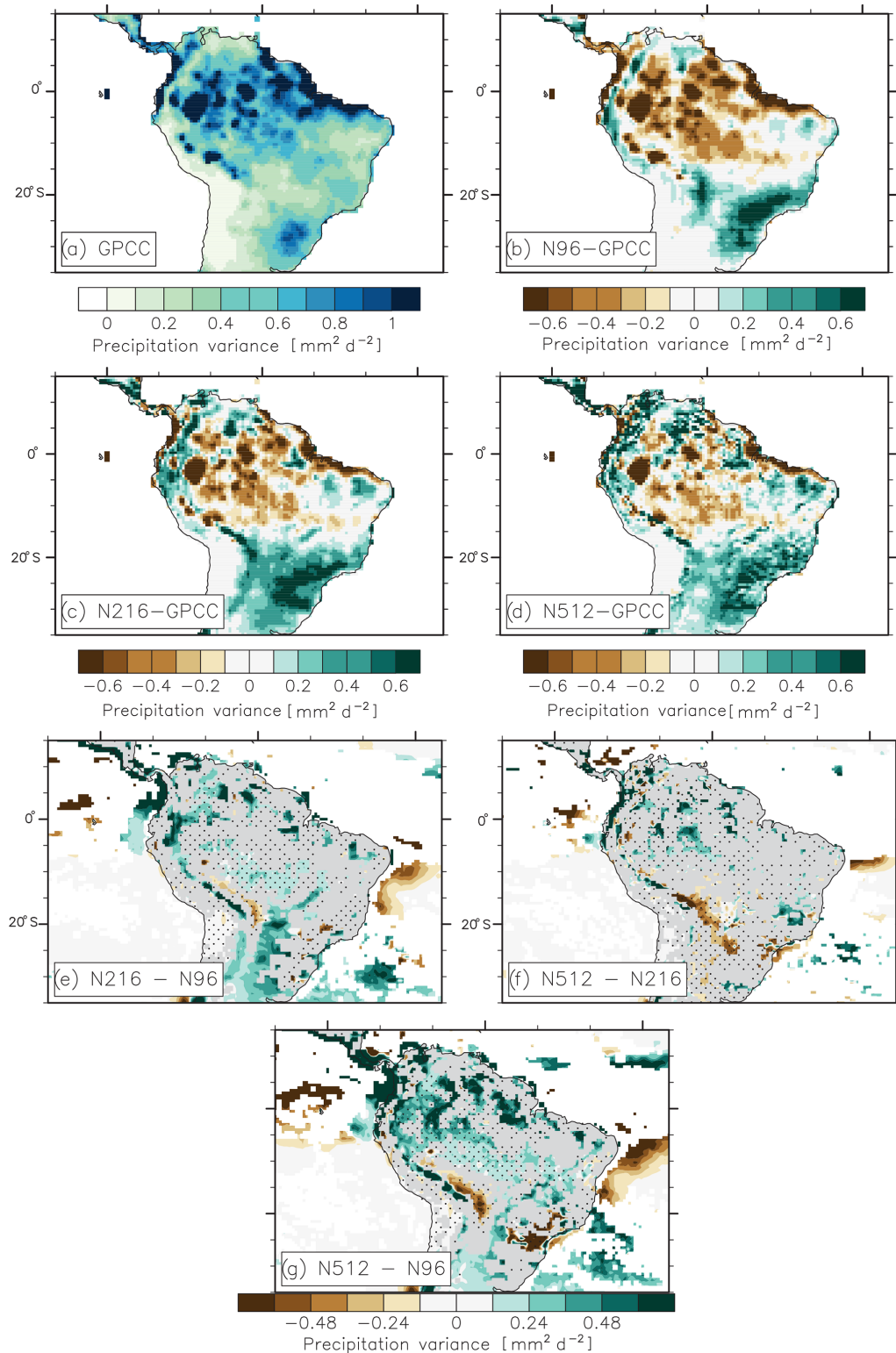
Figure 4. (a) Observed annual-mean precipitation variance (GPCCC; \text{mm}^2 \text{d}^{-2} ), as computed over the period 1982–2014. A linear trend is removed. Bias in annual-mean precipitation variance in (b) N96 (i.e. N96–GPCCC), (c) N216 (i.e. N216–GPCCC), and (d) N512 (i.e. N512–GPCCC). (e) N216–N96, (f) N512–N216, and (g) N512–N96 differences in annual-mean precipitation variance. In (b), (c), and (d), biases are shown when all three members produce a bias that is significant according to an f test and a 95 % confidence level. In (e), (f), and (g), stippling indicates that the bias is improved at the higher rather than at the lower resolution.
