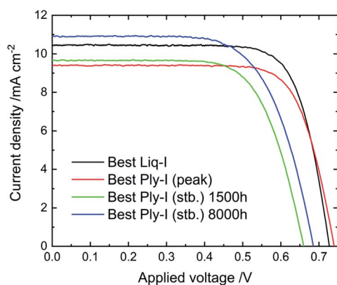
Fig. 2 J - V curves of DSSCs using 5T dye with an aperture of 0.126 cm 2 . Black: best Liq-I DSSC (Cell 1). Red: best Ply-I (peak) DSSC, obtained by drying Cell 1. Green: best Ply-I (stb.) (Cell 2) DSSC measured after 1500 h. Blue: best Ply-I (stb.) DSSC (Cell 2) measured after 8000 h. The Liq-I DSSC is sealed and the Ply-I DSSCs are unsealed.
