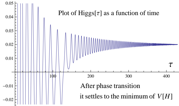
Fig.(1) - After the Big Bang the Higgs field oscillates initially around zero with a large amplitude of the order of the Planck scale. It slowly loses energy to the gravitational field, causing its amplitude to diminish. As it approaches the time or energies of the electroweak scale, it undergoes the phase transition seen in the figure, and then slowly settles to a constant vacuum value v at a stable minimum of the potential.
