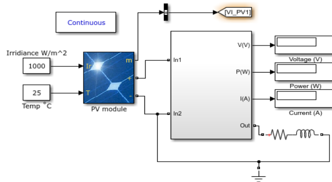
Fig. 5. The model of the simulated monocrystalline PV module tested at dynamic surface temperatures
