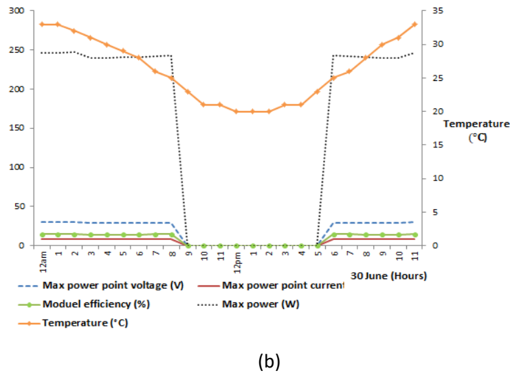
Fig. 9. (a) Power generation from the PV system in Gilgit, North Pakistan, during winter season shows PV system generates the power/voltage efficiently and better than the rest of the regions of Pakistan. (b) Power analysis on the hottest day of 30 th June
