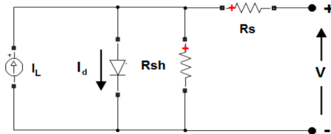
Fig. 2. Illustrates the schematic model of the typical monocrystalline PV cell. The measurements are used to examine the output at different temperatures
