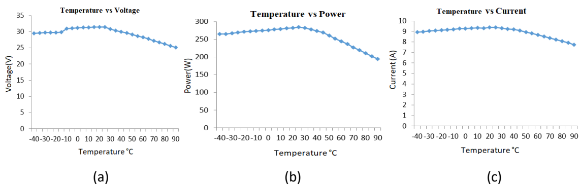
Fig. 4. (a) Illustration of the temperature effects on the voltage. (b) Temperature vs output electrical power from the modelled PV system. (c) Output current variations at different temperature
