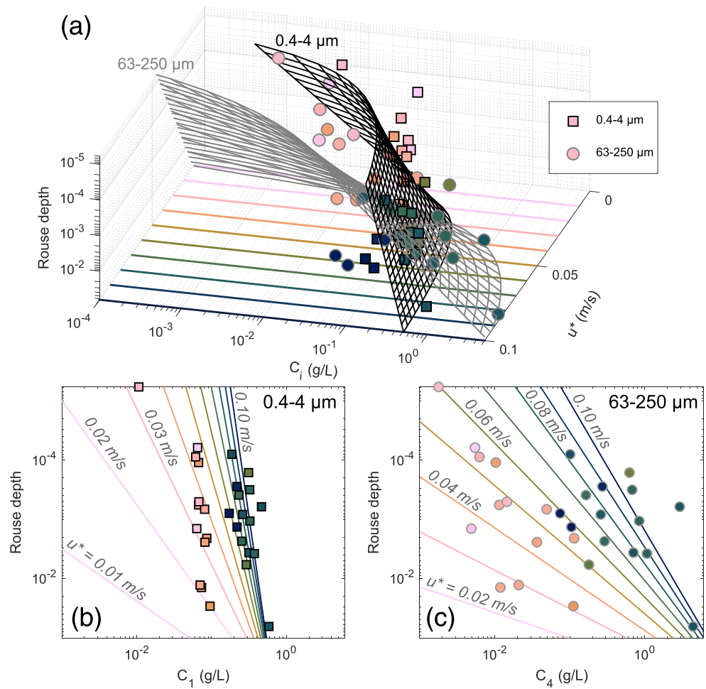
Figure 5. An example of three-dimensional fits to Equation 4 (gridded curved surfaces in panel a) for two grain size fractions of measured Salween River suspended sediment concentrations (circles and squares). Rouse depth ( z_r , as defined in Equation 2) equals 1 at the river bed and 0 at the water surface. Panels b and c show the same fits and sample data in 2-D representation separately for each grain size fraction. The colored lines in the bottom panels are projections (or “slices”) of the three-dimensional gridded surfaces shown in (a) at selected u^* values, as indicated by the colored lines in (a). The sample symbols are also colored according to u^* associated with each sample (Table S1).
