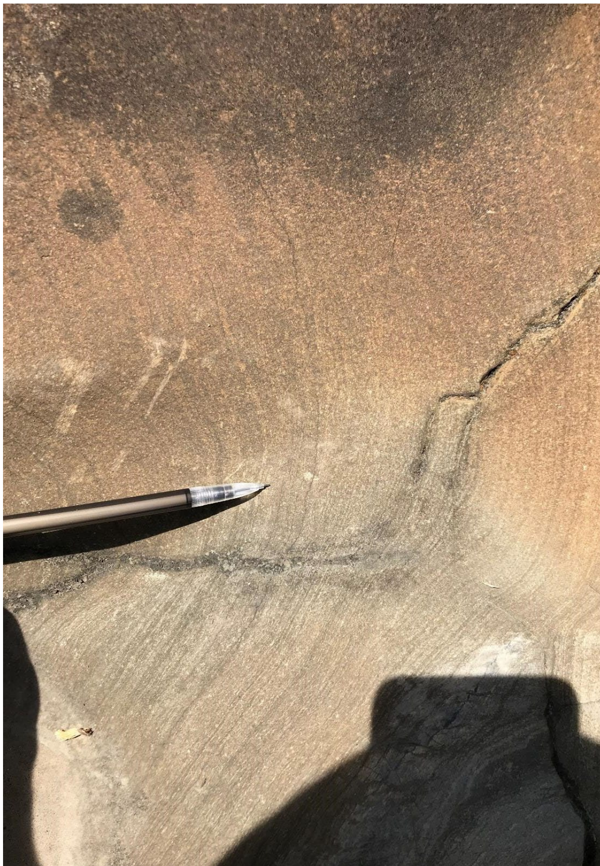
Figure 3.39 The Bleaberry Siltstone Fmt. GR: 27712, 95985. Towards the base of the formation, lamination is much more abundant due to the fine grained nature of the deposits.
