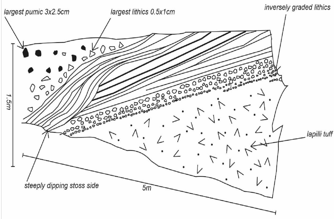
Figure 3.6 Buck Pike Tuff and Clastic Fmt. GR: 26214, 94863. Geological sketch accompanying a field photo of a chute and pool structure with a palaeocurrent of 185° observed in the lapilli tuff member.
