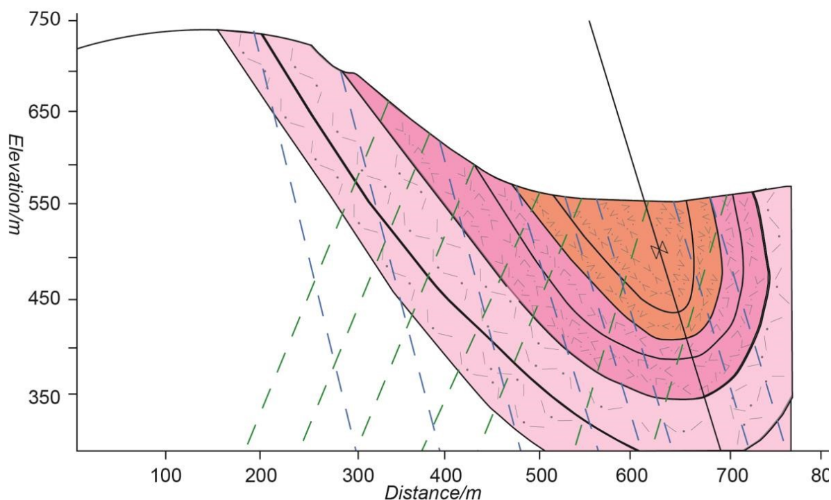
Figure 4.9 A structural cross section through Dow Crag (GR: 26095, 97989 – GR:26698, 97587) displaying an overturned fold with geometries obtained from a stereonet analysis (Fig. 4.2).
