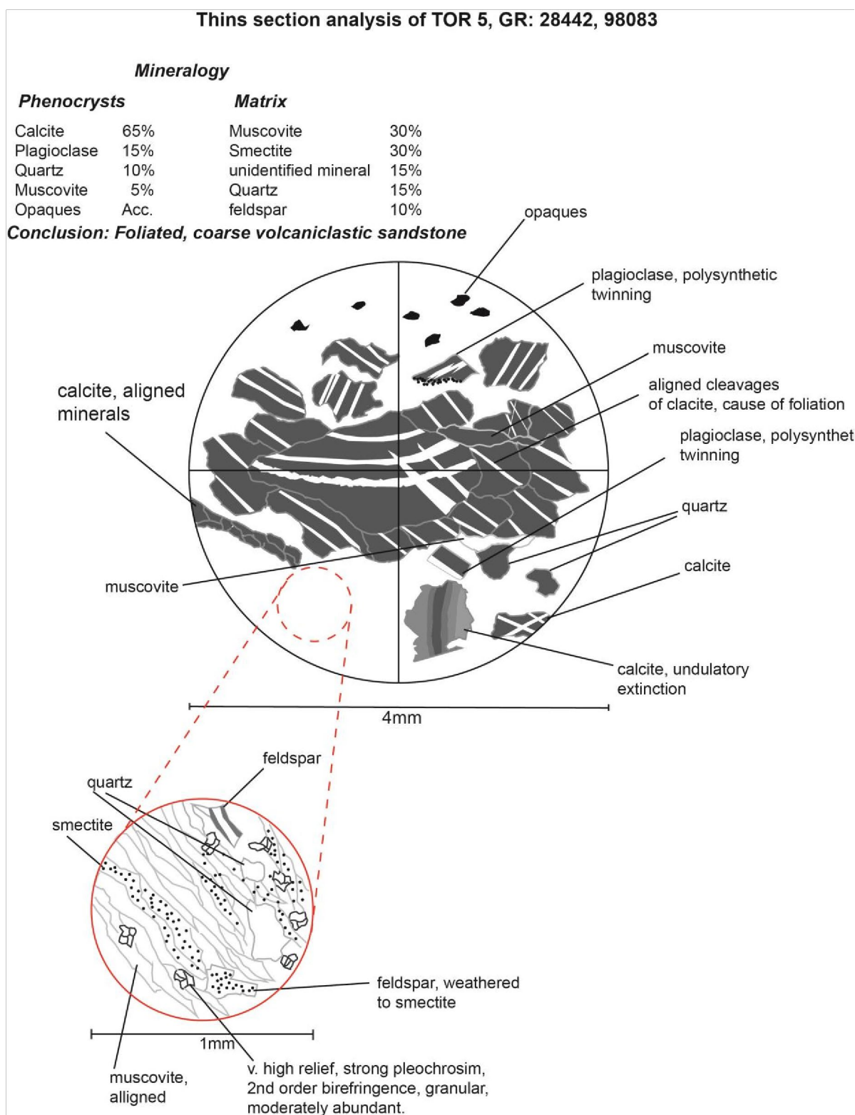
Figure 4.14 Thin section analysis of TOR 5, a foliated volcanoclastic sandstone from the BPTC at Crowberry Haws (GR:28442, 98083). The field of view has been displayed in cross polarised light to highlight alignment of calcite cleavage. Calcite grains hold the highest abundance at 65% and feldspar grains are commonly weathered to smectite.
