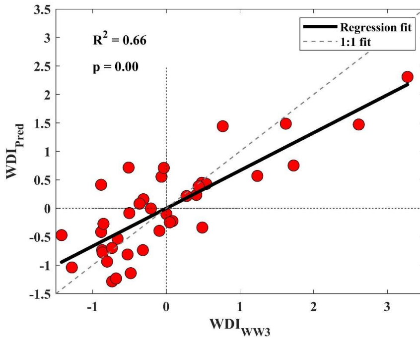
Figure 4.3. WDI WW3 for the winter periods of 1980 to 2018 plotted against WDI Pred predicted using a SMLR model of winter atmospheric indices. The regression fit is shown as the bold line, whilst the 1:1 fit is displayed as the dashed grey line.
