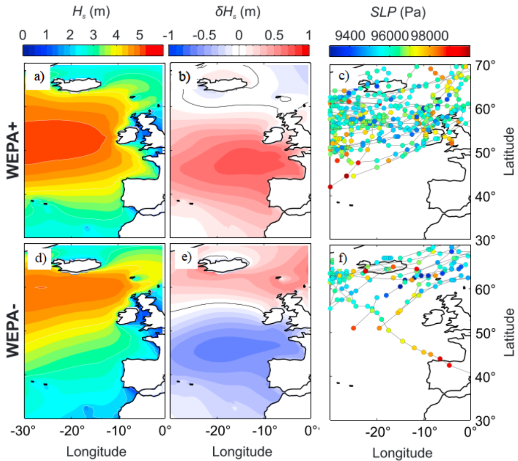
Figure 1.6. Influence of positive and negative WEPA indices on winter-averaged H_s (a, d), corresponding anomaly ( \delta H_s ) (b, e) and storm tracks (c,f), with positive phase and negative phases of each index addressed by averaging the 5 years with the largest and smallest index values over 1950–2016. Superimposed storm tracks over the 5 years with the coloured circles indicating the sea level pressure at the center of the low-pressure system every 6 h. Note that for clarity and to focus on the more severe storms, only identified storms that have a low-pressure center deeper than 96,000 Pa are plotted. By order of decreasing importance, the five winter years considered for each index phase are WEPA+ (2014, 1994, 2001, 2016, and 1977); WEPA- (1992, 1953, 2005, 1976, and 1993), where, for instance, 1977 means the DJFM 1976/1977 winter. Adapted from Castelle et al. (2017).
