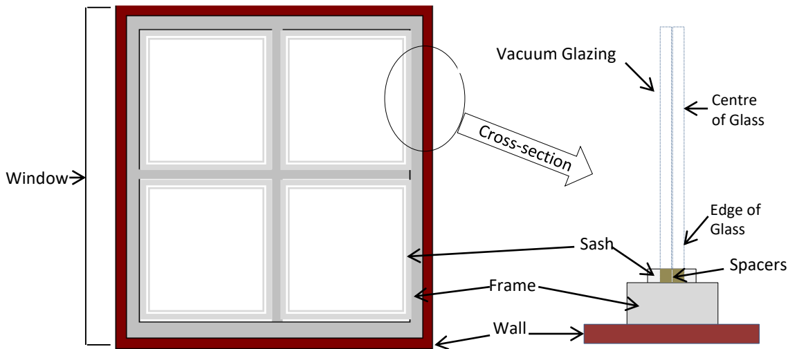
Fig. 1. Window components showing glazing layers separated with spacers and sits in the sash situated on the frame.
