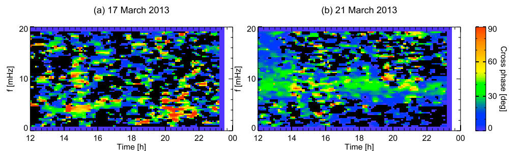
Figure 6. Cross-phase spectra during the (a) main phase and (b) late recovery phase of the St. Patrick's Day 2013 storm from ISLL and GILL B_x ground magnetometer observations.
