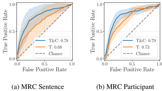
Figure 3: ROC curves for sentence-level (a) and participant (b) classification for the (one-hot) online English Off -medication datasets are included.
