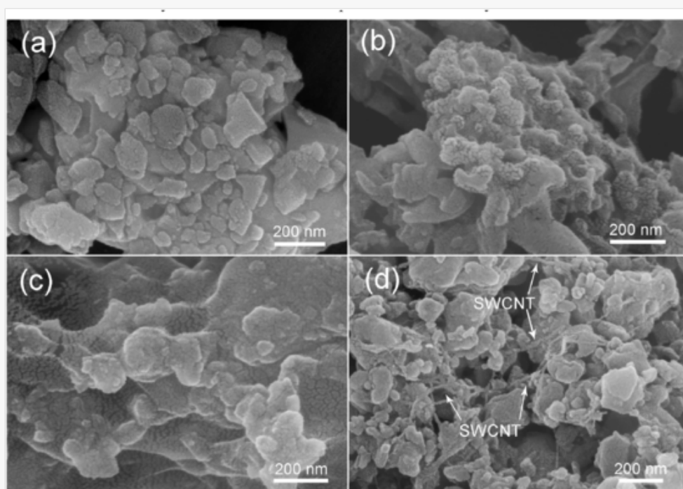
FE-SEM images of (a) TiC, (b) TiC–TiO 2 , (c) TiC–TiO 2 /S and (d) TiC–TiO 2 /SWCNT/S 10.
