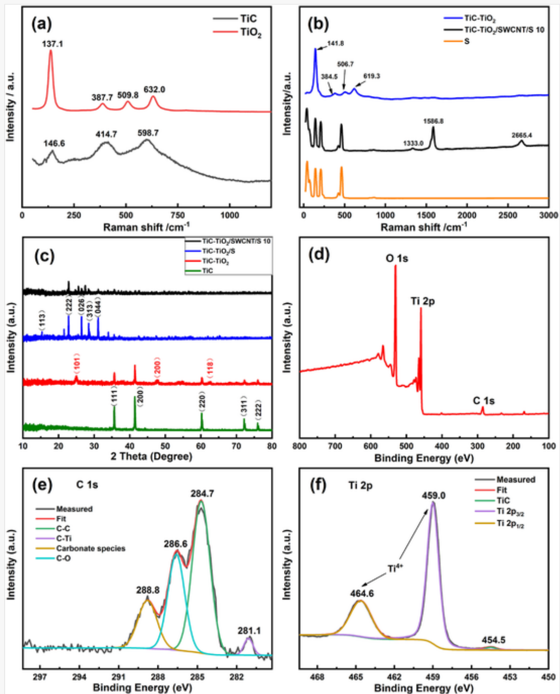
Raman spectra of (a) purchased TiC and TiO 2 ; (b) three distinct materials; (c) XRD patterns of four different materials; XPS spectra of (d) TiC–TiO 2 /SWCNT 10, its (e) C 1s and (f) Ti 2p.
