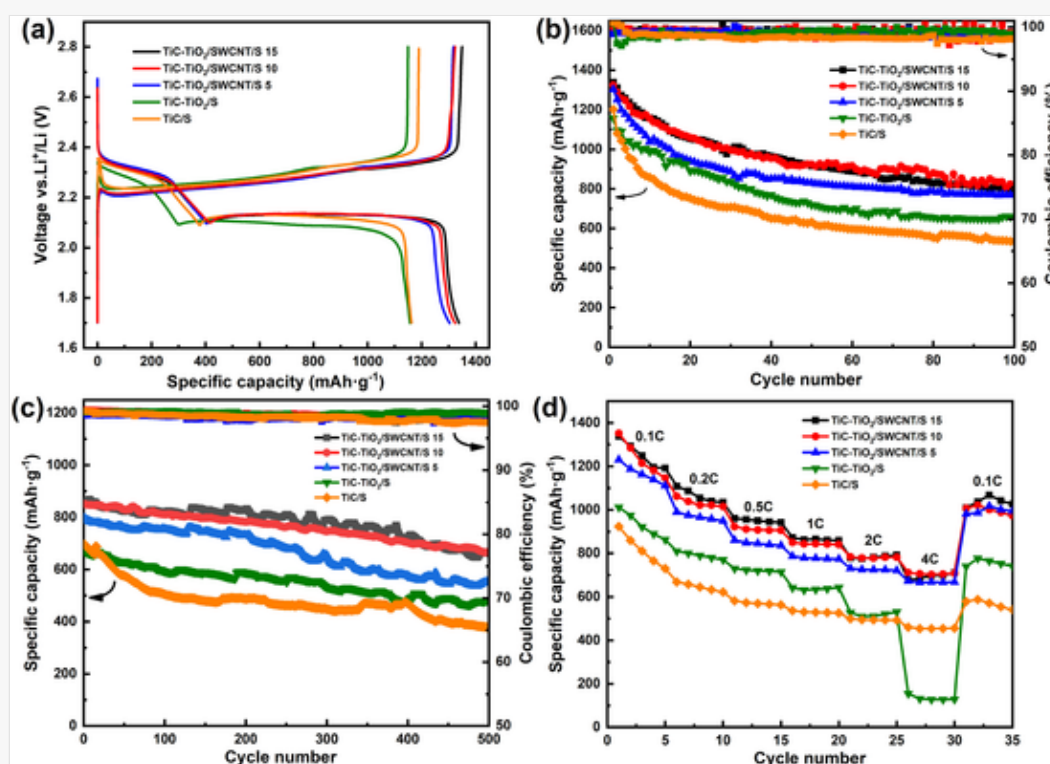
(a) First charge-discharge curves; (b) Charge-discharge performance at 0.1 C, (c) Charge-discharge performance at 1 C large current density and (d) Rate performance from 0.1 C to 4 C of five different cathodes.
