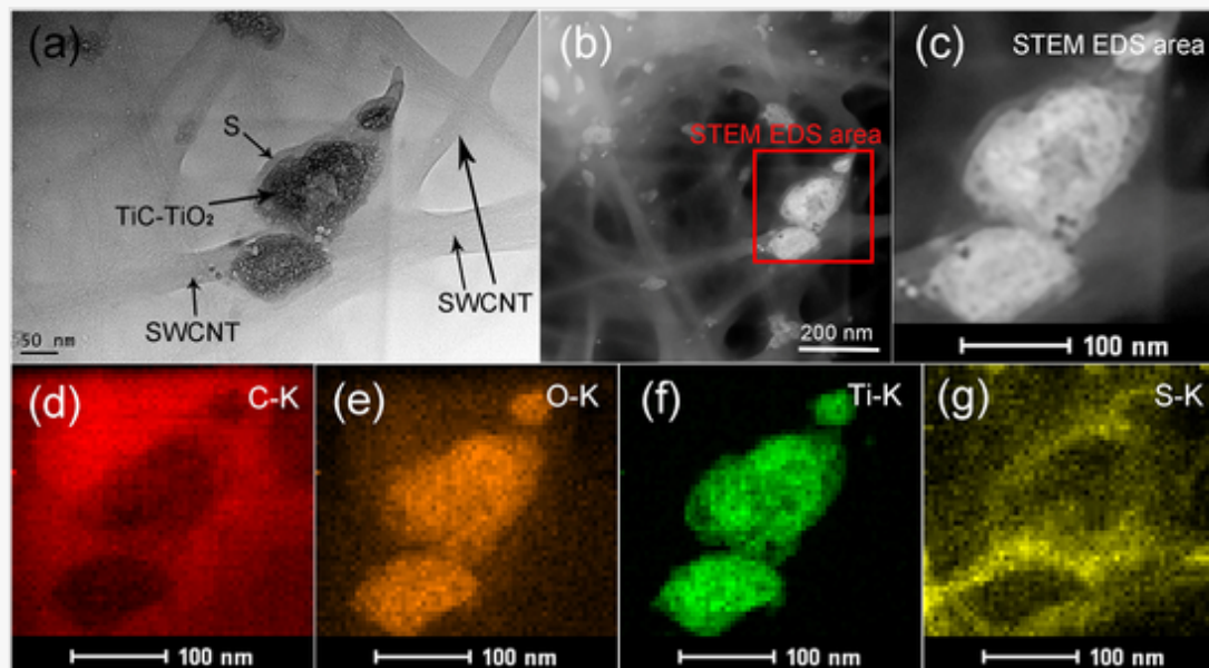
(a) TEM image of TiC–TiO 2 /SWCNT/S 10 composite; (b) STEM image with STEM EDS mapping area and (c) The enlarged view of marked area in (b); STEM EDS elemental mapping of (d) C, (e) O, (f) Ti, (g) S.
