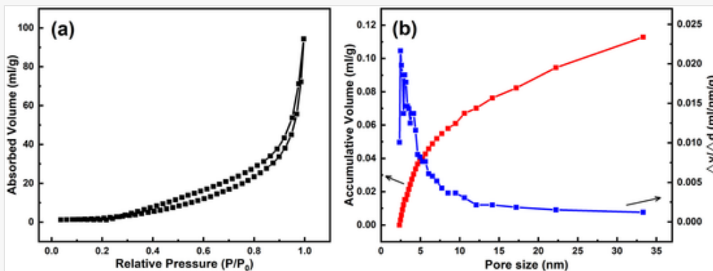
(a) N 2 adsorption-desorption isotherm and (b) pore-size distribution curves of TiC-TiO 2 /SWCNT 10.
