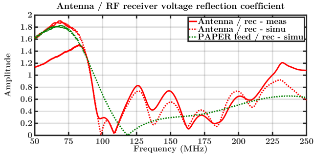
Figure 5. Amplitude of the voltage reflection coefficient at the interface between the antenna output and the receiver input.
