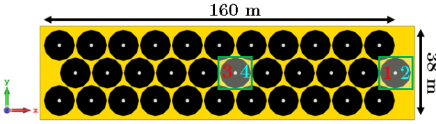
Figure 6. Array configuration used to simulate the mutual coupling in HERA with CST. The red numbers correspond to the ports associated with the X-polarization, and the blue numbers with the Y-polarization.
