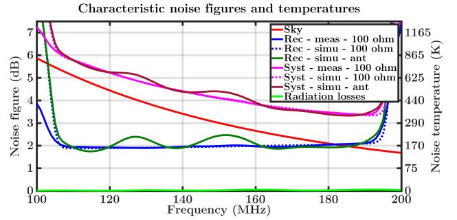
Figure 7. Noise generated by the sky, the radiation losses, and the simulated / measured receivers when terminated by 100\ \Omega or the measured antenna impedance. Combined together, they define the system noise temperature.
