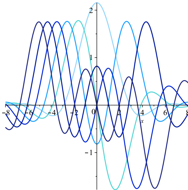
Fig. 3 Transformed Freud functions \varphi_n (with t = \eta = 0 ) for n = 0, \dots, 5 : darker colour denotes greater n (Color figure online)
