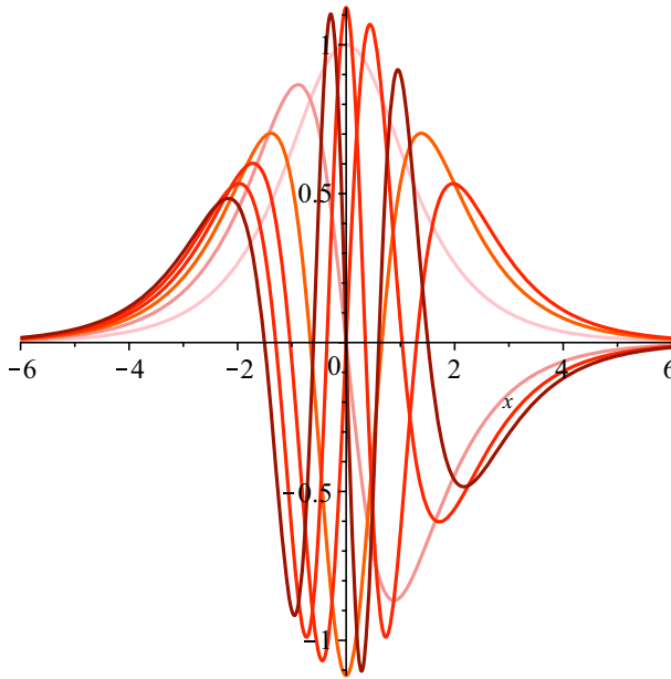
Fig. 2 Transformed Carlitz functions \varphi_n for n = 0, \dots, 5 : darker colour denotes greater n (Color figure online)
