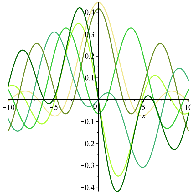
Fig. 1 Transformed Chebyshev functions of the second kind \varphi_n for n = 0, \dots, 5 : darker colour denotes greater n (Color figure online)
