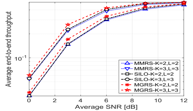
Fig. 10. Throughput with respect to SNR.
