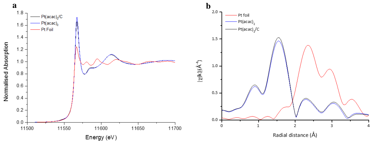
Supplementary Figure 5 – XAS characterisation of the freshly prepared 1wt.% Pt/C-Acetone catalyst. Pt L_{3} -edge a) XANES and b) FT-EXAFS of the freshly prepared 1wt.% Pt(acac) 2 /C catalyst compared with the Pt foil and the Pt(acac) 2 standards.
