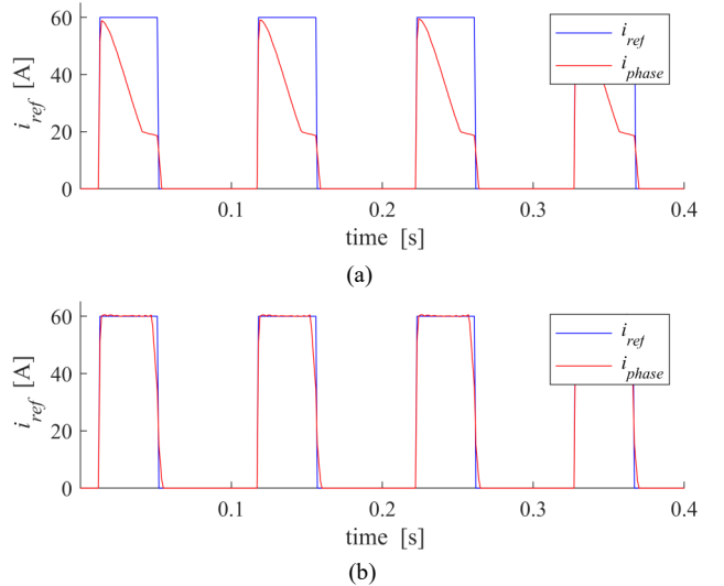
Fig. 3. Operation of the CCS MPC with error in the magnetization surface representation (a) and without (b): blue–current reference; red–flowing current.
