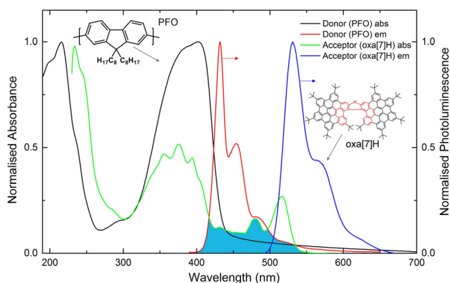
Figure 2. Normalised absorption and photoluminescence ( \lambda_{em} : 385 nm) spectra of thin films of the donor (PFO, thickness, t = 140 nm) and acceptor (oxa[7]H, t = 90 nm) systems used in this work. The overlap between the donor emission and acceptor absorption is highlighted in turquoise.
