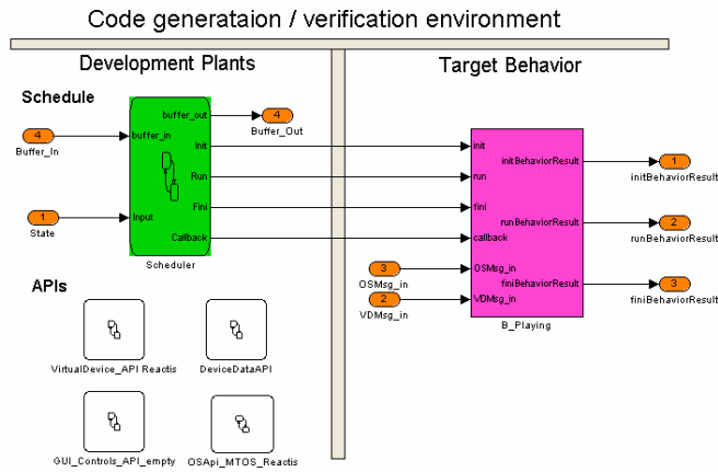
Figure 7. Screen shot of Code generation / verification environment. The behavior under code generation or test inserted into this standard template is the large magenta rectangle at right.
