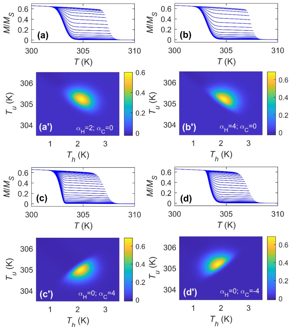
Figure 7. Cooling first order reversal magnetization curves and associated TFORC distributions with \xi_H = T_{t,ST} + 2\text{ K} , \xi_C = T_{t,ST} - 2\text{ K} , \sigma_H = \sigma_C = 0.5\text{ K} and different skewness factor combinations: (a–a') \alpha_H = 2, \alpha_C = 0 , (b–b') \alpha_H = 4, \alpha_C = 0 , (c–c') \alpha_H = 0, \alpha_C = 4 and (d–d') \alpha_H = 0, \alpha_C = -4 .
