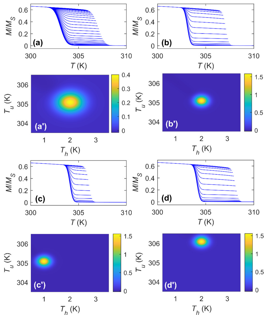
Figure 3. Cooling first order reversal magnetization curves and associated Temperature First Order Reversal Curve (TFORC) distributions with different transformation characteristics: (a–a') \xi_H = T_{t,ST} + 2 K, \xi_C = T_{t,ST} - 2 K and \sigma_H = \sigma_C = 0.5 K, (b–b') \xi_H = T_{t,ST} + 2 K, \xi_C = T_{t,ST} - 2 K and \sigma_H = \sigma_C = 0.25 K, (c–c') \xi_H = T_{t,ST} + 1 K, \xi_C = T_{t,ST} - 1 K and \sigma_H = \sigma_C = 0.25 K and (d–d') \xi_H = T_{t,ST} + 3 K, \xi_C = T_{t,ST} - 1 K and \sigma_H = \sigma_C = 0.25 K. (For all the cases, the skewness factors are zero).
