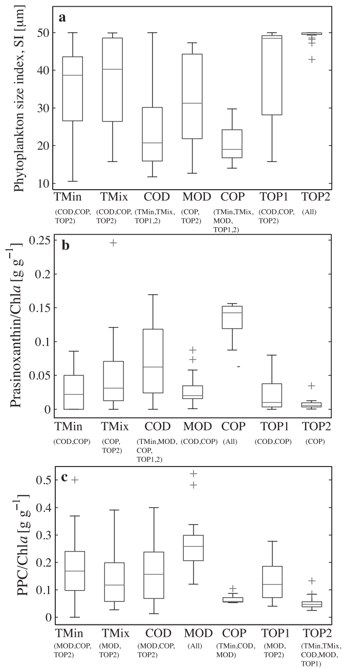
Fig. 7. Boxplots of (a) the phytoplankton size index of Bricaud et al. (2004) calculated from Eq. 5 and the concentration ratios of (b) prasinonanthin and (c) photoprotective carotenoids (PPC) to chlorophyll- a for the seven clusters obtained from HCA of b_{\text{bp}}(\lambda)/a_{\text{p}}(\lambda) . PPC is the sum of alloxanthin, diadinoxanthin, diatoxanthin, zeaxanthin, and alpha- and beta-carotene concentrations. Names of clusters below cluster labels indicate which other cluster means are significantly different as obtained from pairwise t -tests.
