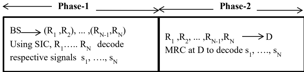
Figure. 11: Illustration of multiple relays assisted transmission within a time slot. Phase I: Transmission from BS to all relay pairs. Phase II: Transmission from all relays to the destination.
