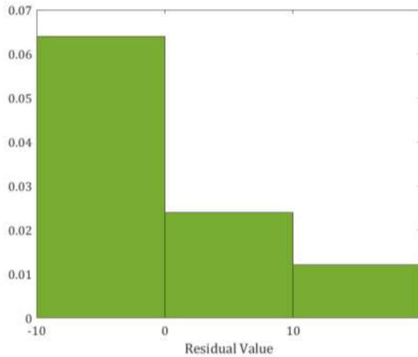
Histogram of Residuals from Linear Regression of ln(AGB – Litter) ~ ln(SfM Volume)
