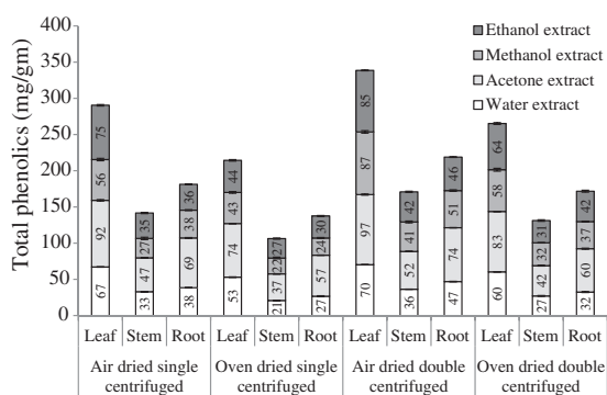
Fig. 1. Total phenolic concentration in boneseed leaf, stem and root extracted using different solvents, drying and centrifuging mechanisms.
