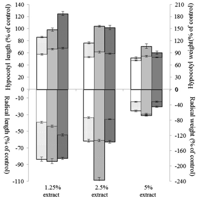
Fig. 4. Effect of different concentrations of boneseed leaf (white), stem (light ash) and root (deep ash) extracts on hypocotyl (upward) and radical (downward) length (plain) and weight (dotted) on A. mearnsii . Data presented as the percentage of control.
