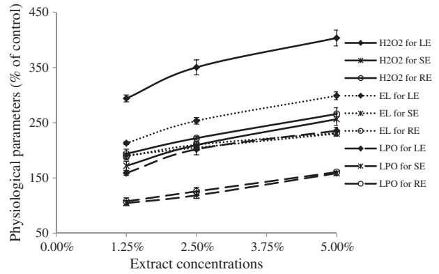
Fig. 9. Impact of boneseed extracts on hydrogen peroxide (H 2 O 2 ), electrolyte leakage (EL) and lipid peroxidation (LPO) of L. sativa . Data presented as the percentage of control. LE = leaf extracts, SE = stem extracts, RE = root extracts.
