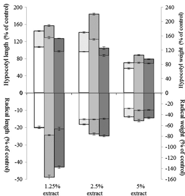
Fig. 5. Effect of different concentrations of boneseed leaf (white), stem (light ash) and root (deep ash) extracts on hypocotyl (upward) and radical (downward) length (plain) and weight (dotted) on L. sativa . Data presented as the percentage of control.
