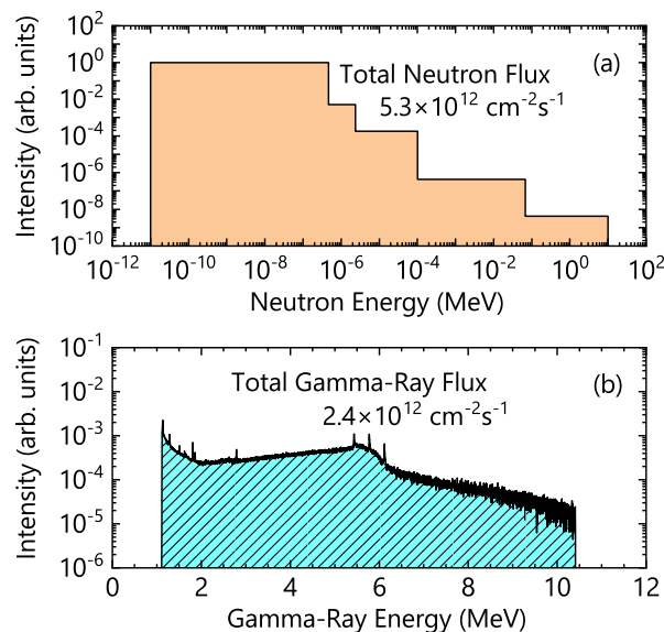
Figure 3: Energy spectra of (a) neutrons and (b) gamma-rays emitted from the planar source (instead of the reactor core) used in the simulation. The total fluxes of neutrons and gamma-rays used for the calculation, corresponding to the values at 5 MW KUR operation, are also indicated, respectively.
