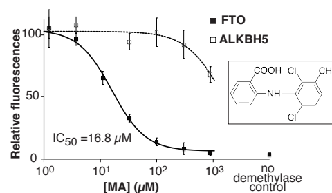
Fig. 5 Inhibition of FTO by meclufenamic acid (MA; inset) detected by FRET-based MazF cleavage assays. MA (0–900 μM) was added to the demethylation samples containing 250 nM FTO (filled square) or 1 μM ALKBH5 (open square), followed by MazF cleavage. The "(m6A)CA" FRET probe was used. The fluorescence intensity obtained from the sample without MA was set to 100. Data are mean ± SD (n = 3).
