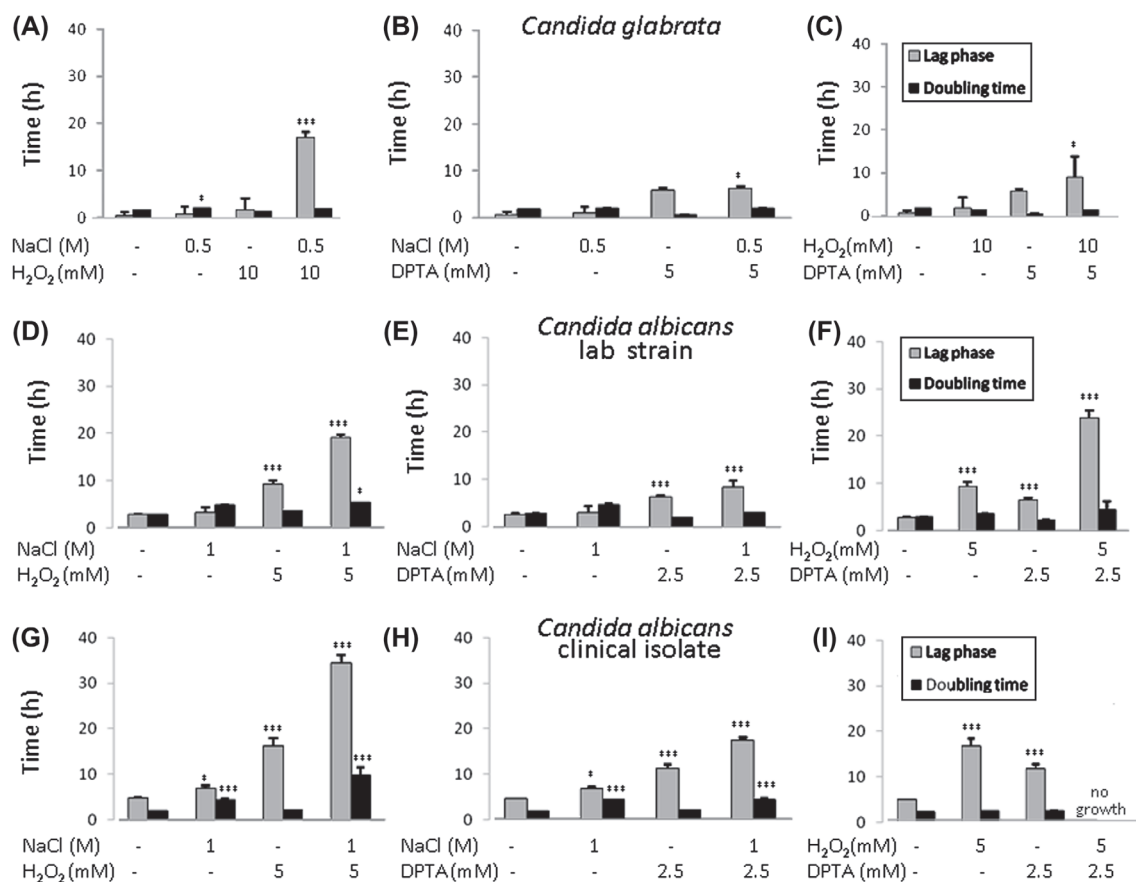
Fig. 4 Effects of medium doses of combinatorial stresses upon the growth of cells in YPDT at 30°C: (A) (B) and (C) C. glabrata ; (D) (E) and (F) C. albicans strain NGY152; (G) (H) and (I) C. albicans isolate SC5314. The lengths of the lag phase and the doubling time were determined mathematically from growth curves as described in Materials and methods : gray bars, length of the lag phase; black bars, doubling time. (A) (D) and (G) Comparison of individual and combinatorial osmotic and oxidative stresses. (B) (E) and (H) Comparison of individual and combinatorial osmotic and nitrosative stresses. (C) (F) and (I) Comparison of individual and combinatorial oxidative and nitrosative stresses. Values were compared to the no stress controls and significant increases highlighted: * P \leq 0.05 ; ** P \leq 0.01 ; *** P \leq 0.001 .
