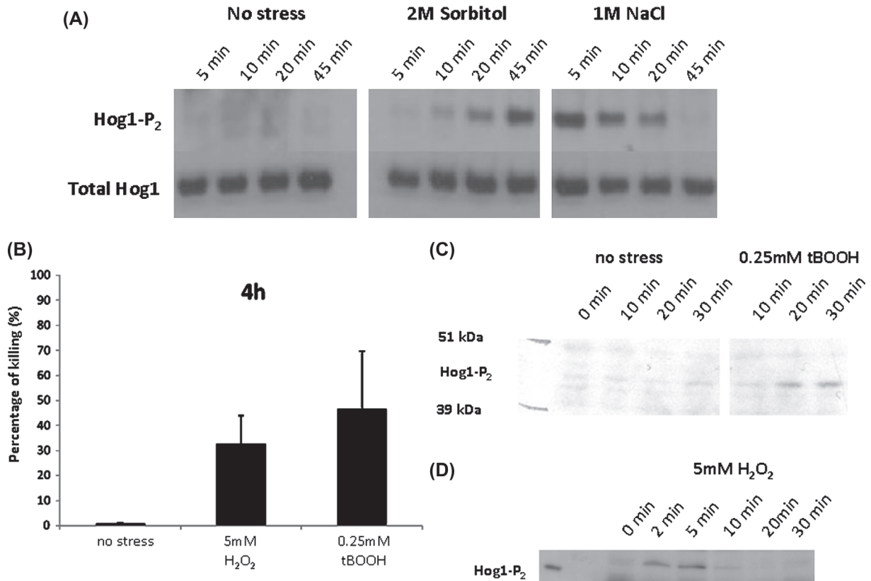
Fig. 1 Comparison of the effects of specific stressors upon Candida albicans and Candida glabrata cells grown in YPDT at 30°C. (A) Impact of 2 M sorbitol and 1 M NaCl upon the dynamics of Hog1 phosphorylation in C. glabrata : upper panels, Western blots probed with a phospho-specific antibody against Hog1; lower panels, Western blots probed with an anti-Hog1 antibody that detects total Hog1 (loading control). (B) Impact of 4 h exposure to 5 mM H 2 O 2 and 0.25 mM tBOOH upon C. albicans killing as quantified by propidium iodide staining and FACS analysis. (C) Dynamics of Hog1 phosphorylation in C. albicans following exposure to 0.25 mM tBOOH as assayed by Western blotting. (D) Dynamics of Hog1 phosphorylation in C. albicans following exposure to 5 mM H 2 O 2 .
