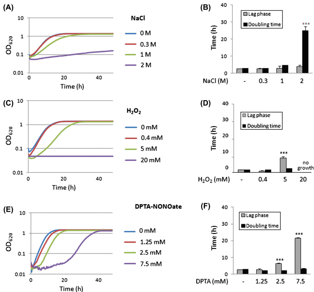
Fig. 3 Dose-dependent effects of osmotic, oxidative and nitrosative stresses upon the growth of Candida albicans in YPDT at 30°C. The lengths of the lag phase and the doubling time were determined mathematically from growth curves as described in Materials and Methods. (A) Effects of NaCl upon growth. (B) Effects of NaCl upon the length of the lag phase and the doubling time. (C) Effects of H 2 O 2 upon growth. (D) Effects of H 2 O 2 upon the length of the lag phase and the doubling time. (E) Effects of DPTA-NONOate upon growth. (F) Effects of DPTA-NONOate upon the length of the lag phase and the doubling time. Values were compared to the no stress controls and significant increases highlighted: * P \leq 0.05 ; ** P \leq 0.01 ; *** P \leq 0.001 . This Figure is reproduced in color in the online version of Medical Mycology .
