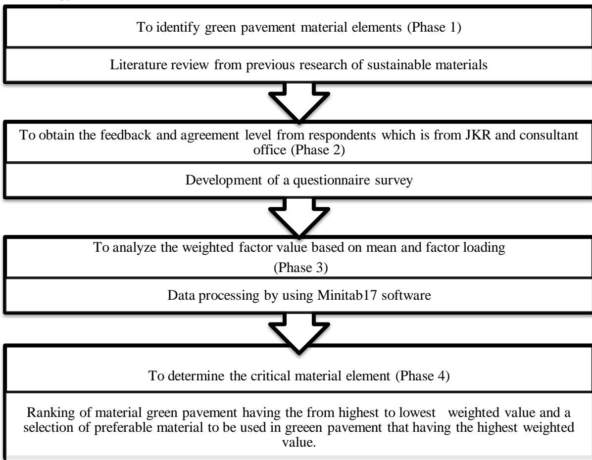
Figure 1. Methodology flowchart
