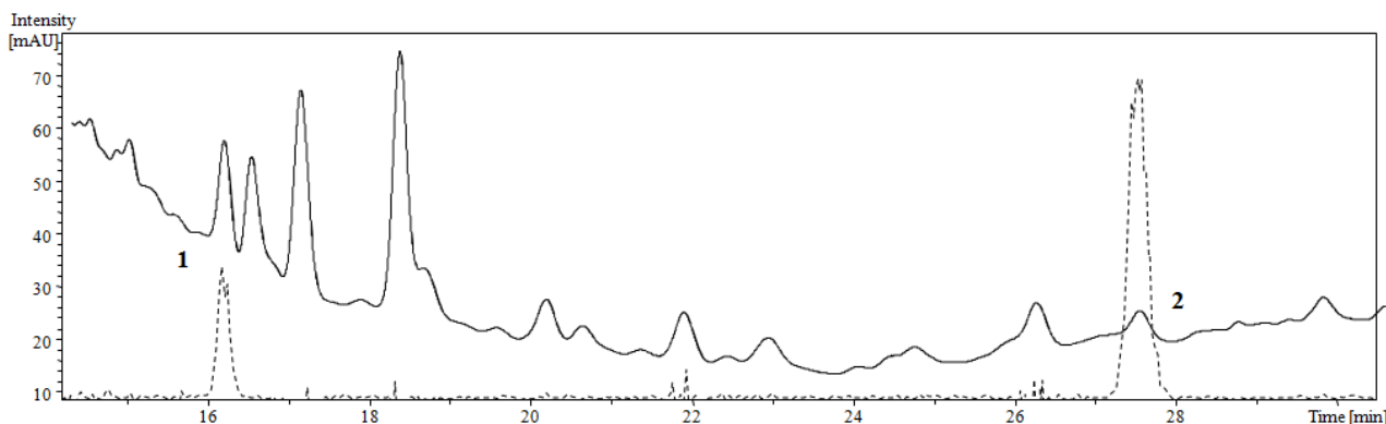
Fig. 2. UV/Vis chromatograms of Vranac wine (—) and standard solution (---) recorded at 306 nm for separation and quantification of stilbenes. Peak assignment: (1) trans -resveratrol-3-glucoside, t_R = 16.2 min; (2) trans -resveratrol, t_R = 27.5 min
