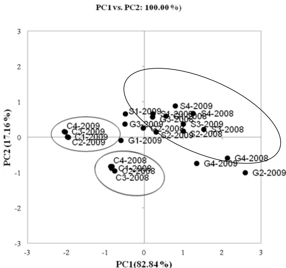
Fig. 4. Classification of Vranac wines produced with different fermentation tanks (classical, Sifa and Ganimede) during 2008 and 2009 and applying different enological additives (enzyme, oak chips and grape tannins) analysed in function of PC1 and PC2, based on resveratrol and resveratrol-3-glucoside variables. Labels of the wines correspond to those in Table 2.
