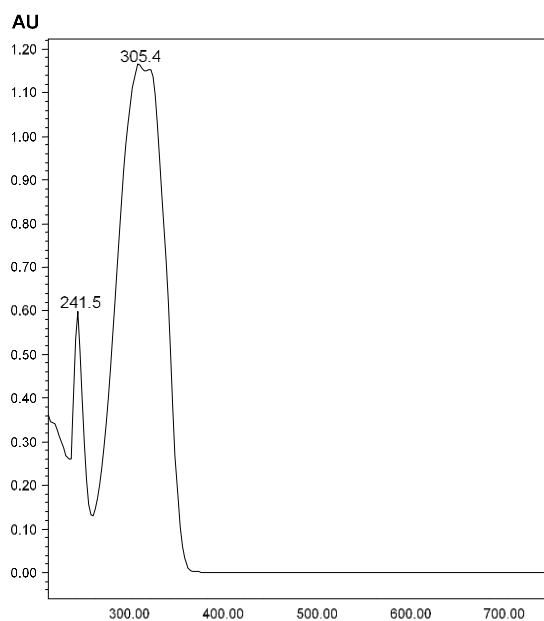
Fig. 1. UV/Vis spectra of resveratrol-glycoside recorded at 200 to 750 nm
