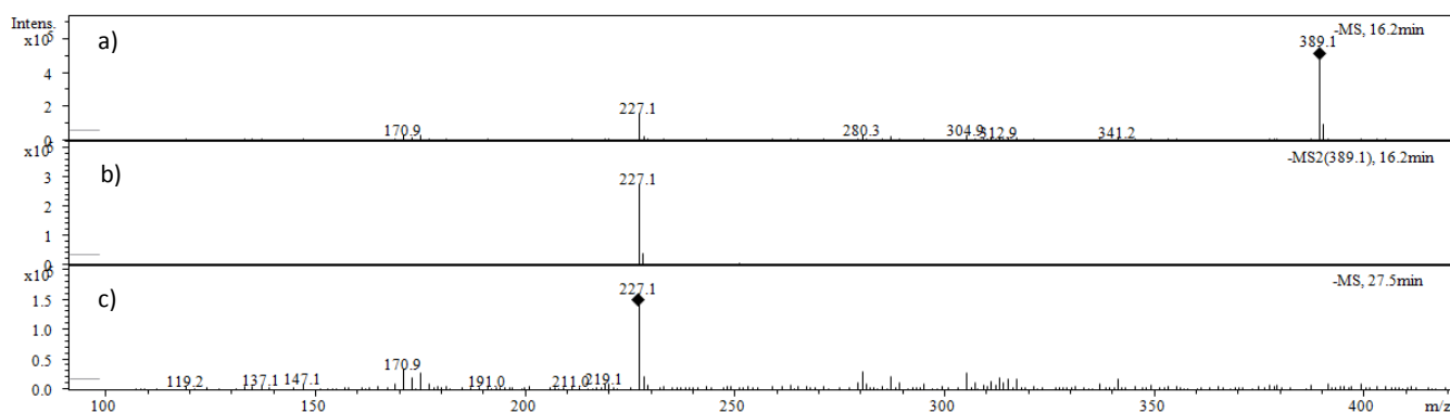
Fig. 3. MS/MS spectra of trans -resveratrol-3-glucoside (a, b) and trans -resveratrol (c) obtained in negative ion mode
