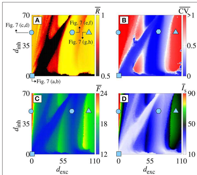
FIGURE 6 | (A) \bar{R} , (B) \overline{CV} , (C) \bar{F} , and (D) \bar{I}_s in the parameter space d_{exc} \times d_{inh} for g_{exc} = 0.8 nS and g = 6 . Symbols in d_{exc} \times d_{inh} correspond to d_{exc} = d_{inh} = 0 ms (cyan square), d_{exc} = 0 ms and d_{inh} = 50 ms (cyan circle), d_{exc} = 70 ms and d_{inh} = 50 ms (cyan hexagon), and d_{exc} = 110 ms and d_{inh} = 50 ms (cyan triangle).
