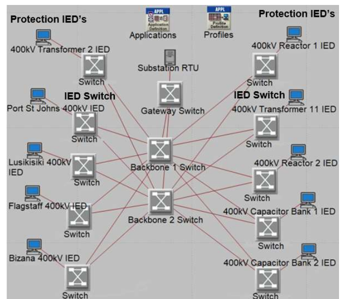
Fig. 2 OPNET Substation Communication Network Model
