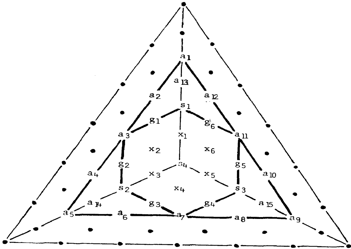
Figure 11: Constructing the C^2 solution.
