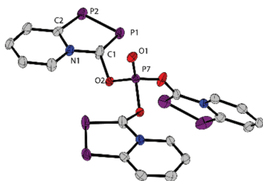
Fig. 1 Crystal structure of compound 4. Anisotropic thermal displacement ellipsoids are shown at the 50% probability level. Hydrogen atoms and the solvent molecules are omitted for clarity reasons. Average interatomic distances (Å) summarized in Table 1.
