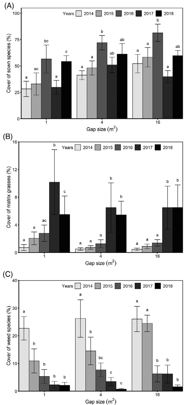
Figure 1. Cover scores (mean \pm SE) of sown (A), matrix (B), and weed species (C) in the establishment gaps from 2014 to 2018 in the Hortobágy National Park. Letters indicate significant differences in the cover scores between the years within different gap sizes (GLMM and least significant difference test, p < 0.05 ).
