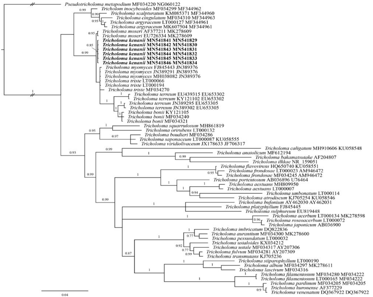
Fig. 32. Phylogeny of Tricholoma species showing the placement of T. kenanii , reconstructed from a concatenated ITS–LSU data-set. The topology is the result on Bayesian inference performed with MrBayes. Sequences of the newly described species are highlighted in boldface. Only BIPP >0.75 are shown.
