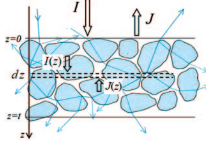
Fig. 2. – Positive ( I ) and negative ( J ) flowing fluxes in an inhomogeneous layer of thickness t . The random propagation of a single light ray subjected to multiple refractions and reflections is also sketched (cyan lines).
