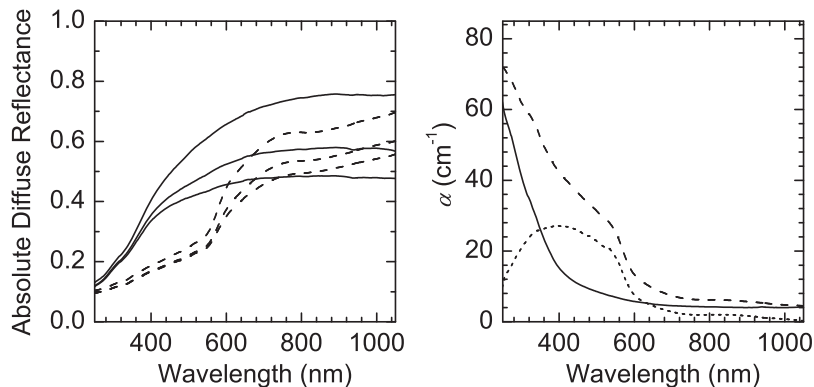
Fig. 4. – R_w , R_b and R_\infty spectra of the area of the SA named 2 (solid lines) and 3 (dashed lines) (left panel) and recovered intrinsic absorption coefficients (right panel). The short-dashed curve is the difference between absorption coefficients of areas 3 and 2.
