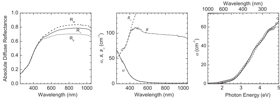
Fig. 3. – R_w , R_b and R_\infty spectra of the folio 11 verso of the CFB (left panel). \alpha (measured and estimated below 350 nm by using eq. (9)), s and s_\infty (central panel). The experimental and theoretical absorption coefficients of cellulose fibres in the measured spot (right panel).
