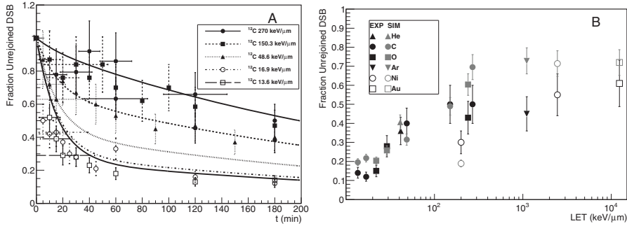
Fig. 3. – A: Experimental data (symbols) and predictions (lines) of DSB rejoining over time after irradiation of CHO-K1 cells with carbon ions at different energies ( \tau_{\text{fast}} = 9 \pm 1 min, \tau_{\text{slow}} = 220 \pm 16 min); B: Remaining fractions of DSB 3 h after ion irradiation of CHO-K1 cells, experimental data (black) and model predictions (grey), half-lives are obtained by fitting an independent data set ( \tau_{\text{fast}} = 11 \pm 2 min, \tau_{\text{slow}} = 428 \pm 126 min). For details about irradiation doses see the original manuscript. Adapted with permission from Tommasino et al. [7].
