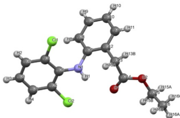
Figure 5. The 3D structure of ethyl diclofenac.
