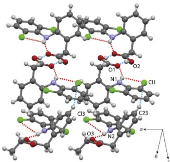
Figure 13. Hydrogen bonding of EDDA.
