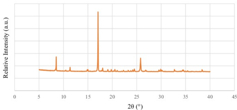
Figure 4. Diffractogram of ethyl diclofenac.
