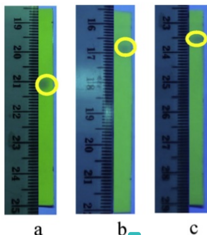
Figure 4. Chromatogram of ethyl diclofenac on silica gel 60 F-254 using three types of mobile phases: a) n-hexane: ethyl acetate (8:1), b) ethanol: ethyl acetate (2:3), and c) toluene: acetone (1:2)—under UV 254 nm lamp.
