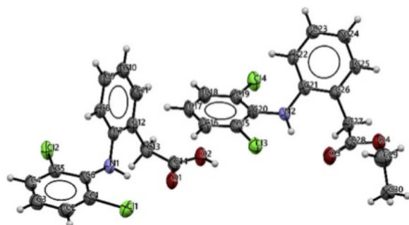
Figure 12. The 3D structure of the EDDA cocrystal.
