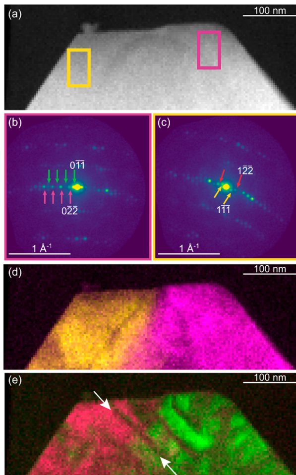
Fig. 10 (a) STEM image UiO-66(Hf) particle with high defect density, where integrated electron diffraction patterns (b, c) were selected in magenta and yellow. (d) Composite virtual dark-field (VDF) image formed using integration windows centered on parent reflections, magenta in b and yellow in c. (e) Composite VDF image formed using integration windows centered on superlattice reflections, green in b and red in c. Reproduced with permission. 111 Copyright 2020, American Chemical Society.
