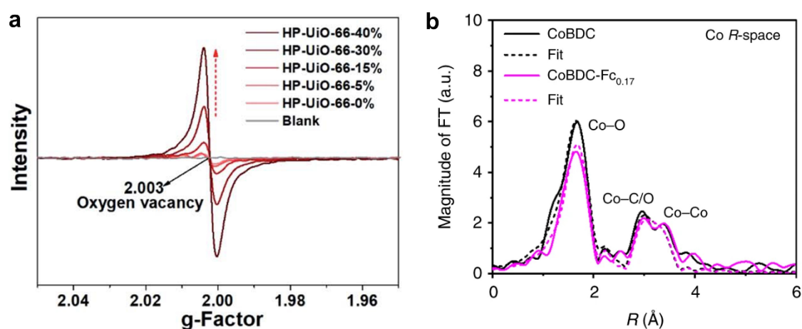
Fig. 7 (a) EPR spectra of HP-UiO-66. Reproduced with permission. 11 Copyright 2020, Royal Society of Chemistry. (b) Fourier transformed EXAFS spectra of CoBDC and CoBDC-Fc 0.17 . Reproduced with permission. 33 Copyright 2019, Springer Nature.
