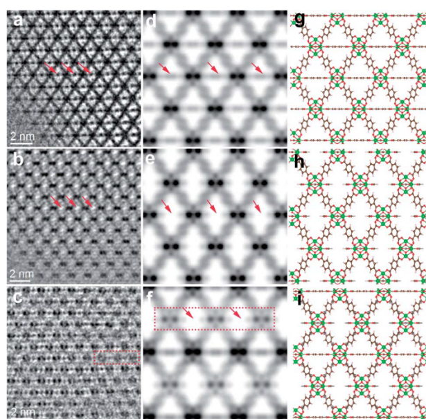
Fig. 9 HRTEM images of (a) UiO-66 and (b) missing-linker defect and (c) missing-cluster defect regions of UiO-66(1d) along the [110] zone axis; (d-f) and (g-i) represent relative simulated potential maps and structural models, respectively. Reproduced with permission. 29 Copyright 2020, Royal Society of Chemistry.
