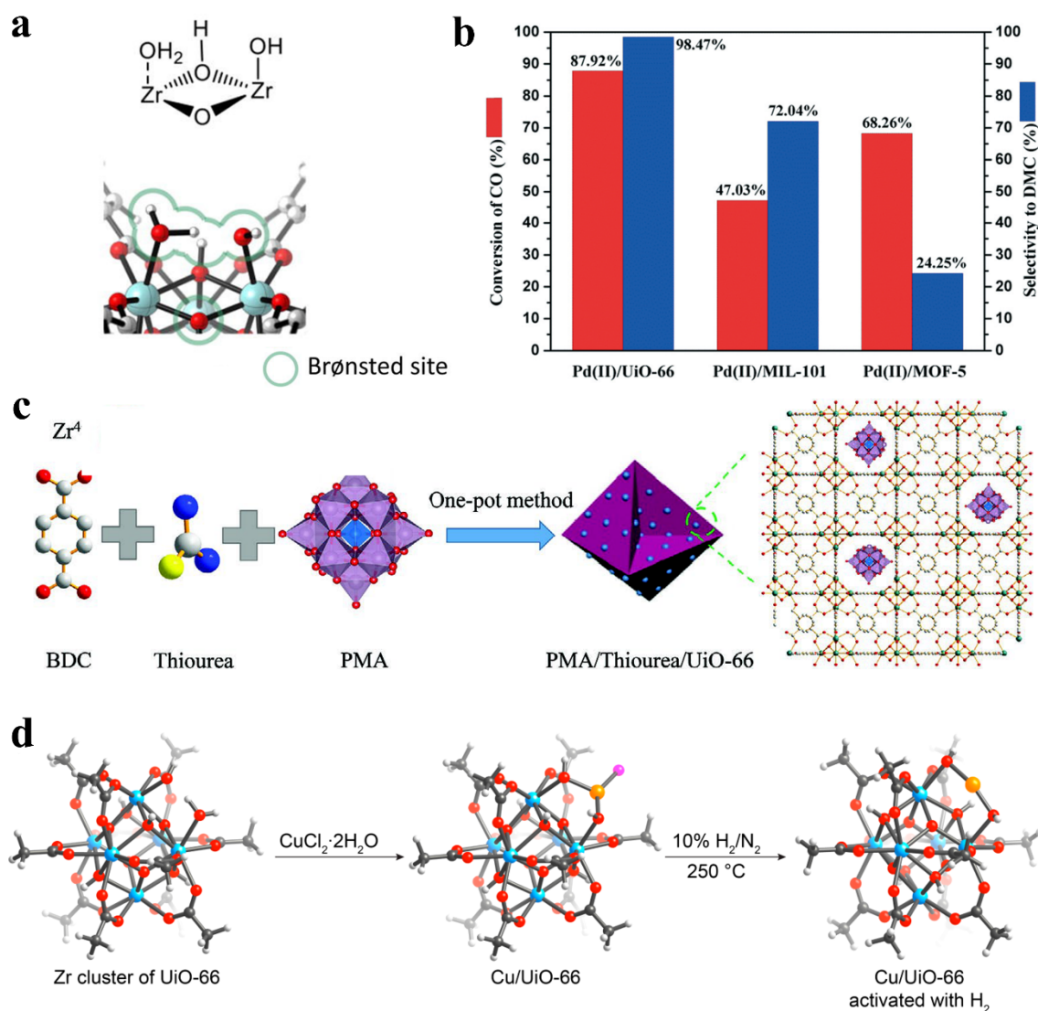
Fig. 11 (a) A calculated configuration structure of three water molecules and a coordinatively unsaturated Zr-brick in defective UiO-66. Reproduced with permission. 20 Copyright 2017, Elsevier. (b) The conversion of CO and selectivity to DMC over Pd(II)/MOFs catalysts for CO esterification to DMC. Reproduced with permission. 27 Copyright 2020, Royal Society of Chemistry. (c) Preparative route for POMs/defective MOFs composites. Reproduced with permission. 37 Copyright 2020, Wiley-VCH. (d) The calculated structures of defective UiO-66 and a Cu/UiO-66 catalyst before and after activation with H 2 . Atom labeling: C, black; O, red; Cl, pink; Cu, orange; Zr, blue. H: light gray. Reproduced with permission. 39 Copyright 2019, American Chemical Society.
