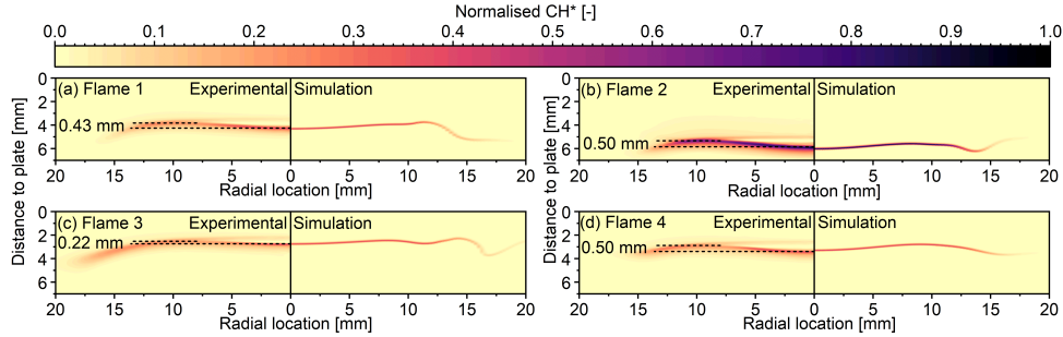
Figure 2: Normalised \text{CH}^* profiles obtained from experiments by recording the \text{CH}^* chemiluminescence (left-hand panes) and the 2D simulations (right-hand panes). The dotted lines mark the points used to calculate the difference in vertical position, \epsilon .
