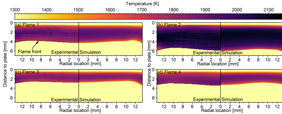
Figure 4: Cross sections of temperature profiles from thin filament pyrometry experiments (left-hand panes) and 2D simulations (right-hand panes). The average of three repeat measurements are reported.
