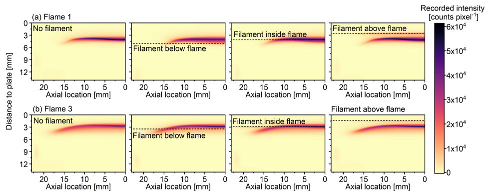
Figure 3: Recorded \text{CH}^* chemiluminescence from the undisturbed flames (left-hand panes) and from the flames with a SiC filament inside their centre at different distances from the plate.
