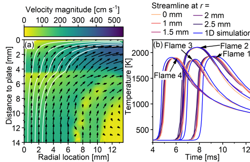
Figure 6: (a) 2D velocity-streamline plot for Flame 1 and (b) temperature-residence time plot for all flames. The abrupt change in the streamlines occurs at the flame front (left panel).
