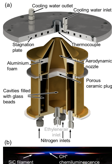
Figure 1: (a) Rendered CAD drawing of the in-house developed premixed burner and water cooled stagnation surface. (b) Photograph of the SiC filament inside the premixed stagnation stabilised flat flame.
