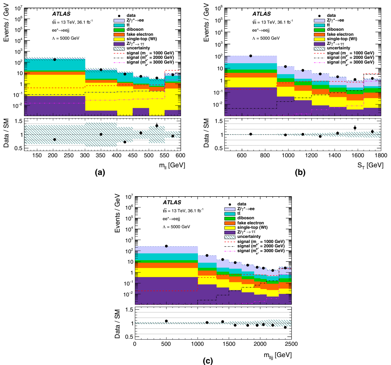
Fig. 3 The distributions of a m_{\ell\ell} , b S_T , and c m_{\ell jj} used to discriminate the signal from background processes in the eejj channel. The distributions are shown after applying the preselection criteria. The background contributions are constrained using the CRs. The signal models assume \Lambda = 5 TeV. The last bin includes overflow events (the
