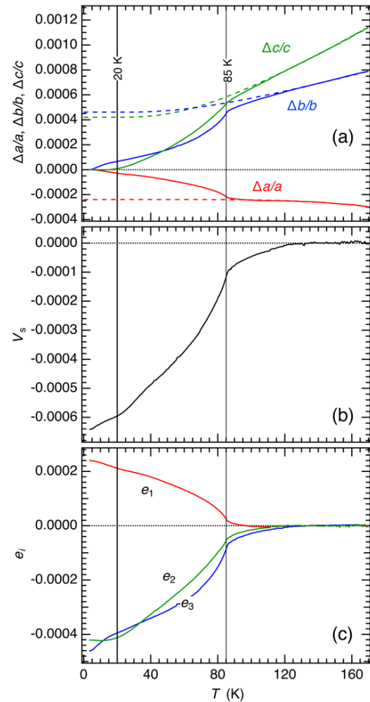
Figure A4. (a) High resolution linear thermal expansion data for NdMnO 3 reported in Meier [64] and Berggöld et al [66]. Dashed lines are baselines, representing linear expansion of the high symmetry structure, obtained by first fitting Equation A1 to data in the temperature interval 123-190 K for \Delta c/c which gave \Theta_s = 104.7 K. This value of \Theta_s was fixed when fitting to the data for \Delta b/b in the same temperature interval. The baseline for \Delta a/a was fit to data in the temperature interval 120-170 K and had \Theta_s = 369 K.
