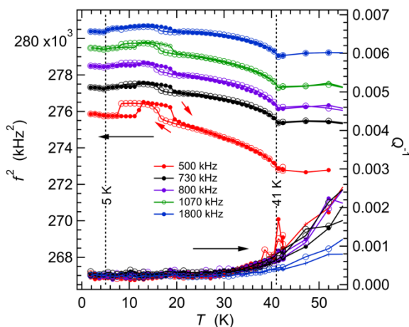
Figure 4. Variation of f^2 (a) and Q^{-1} (b) at low temperatures from fitting of five resonance peaks in RUS spectra collected from the single crystal of \text{GdMnO}_3 during cooling (open circles), followed by heating (filled circles) in the Teslatron cryostat. Absolute values of f^2 have been scaled arbitrarily along the y -axis to allow for easy comparison of the trends which they each display. Listed frequencies refer to the approximate frequency of each resonance at room temperature.
