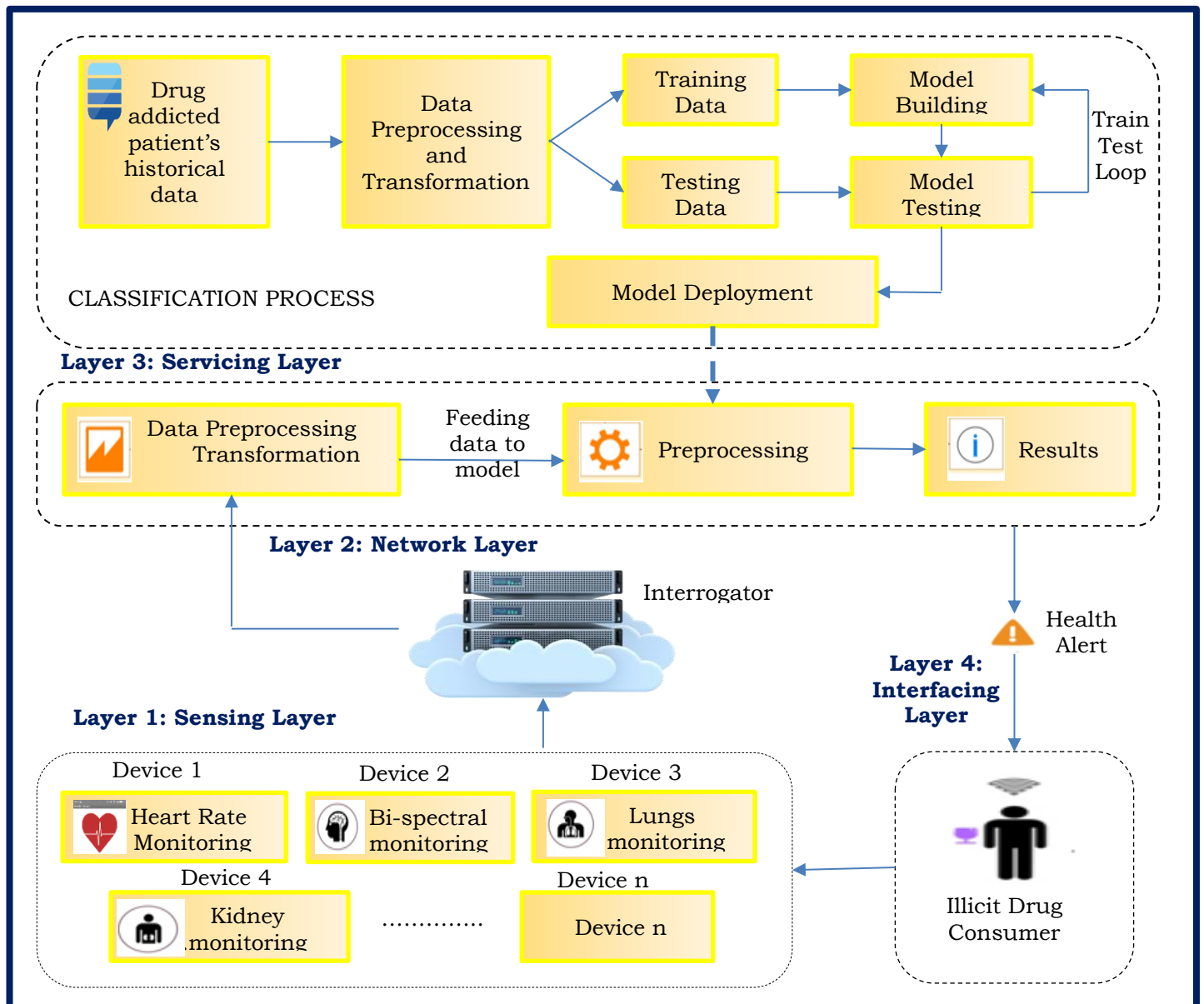
Figure 2. SOA based EHS for Alcohol Addiction Prediction
