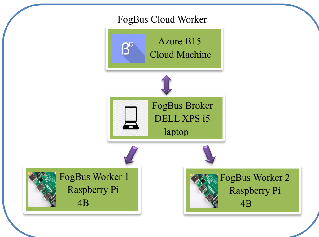
Figure 14. Evaluation Testbed
