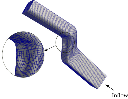
Fig. 2: 3D duct flow with perturbed inward bump.
