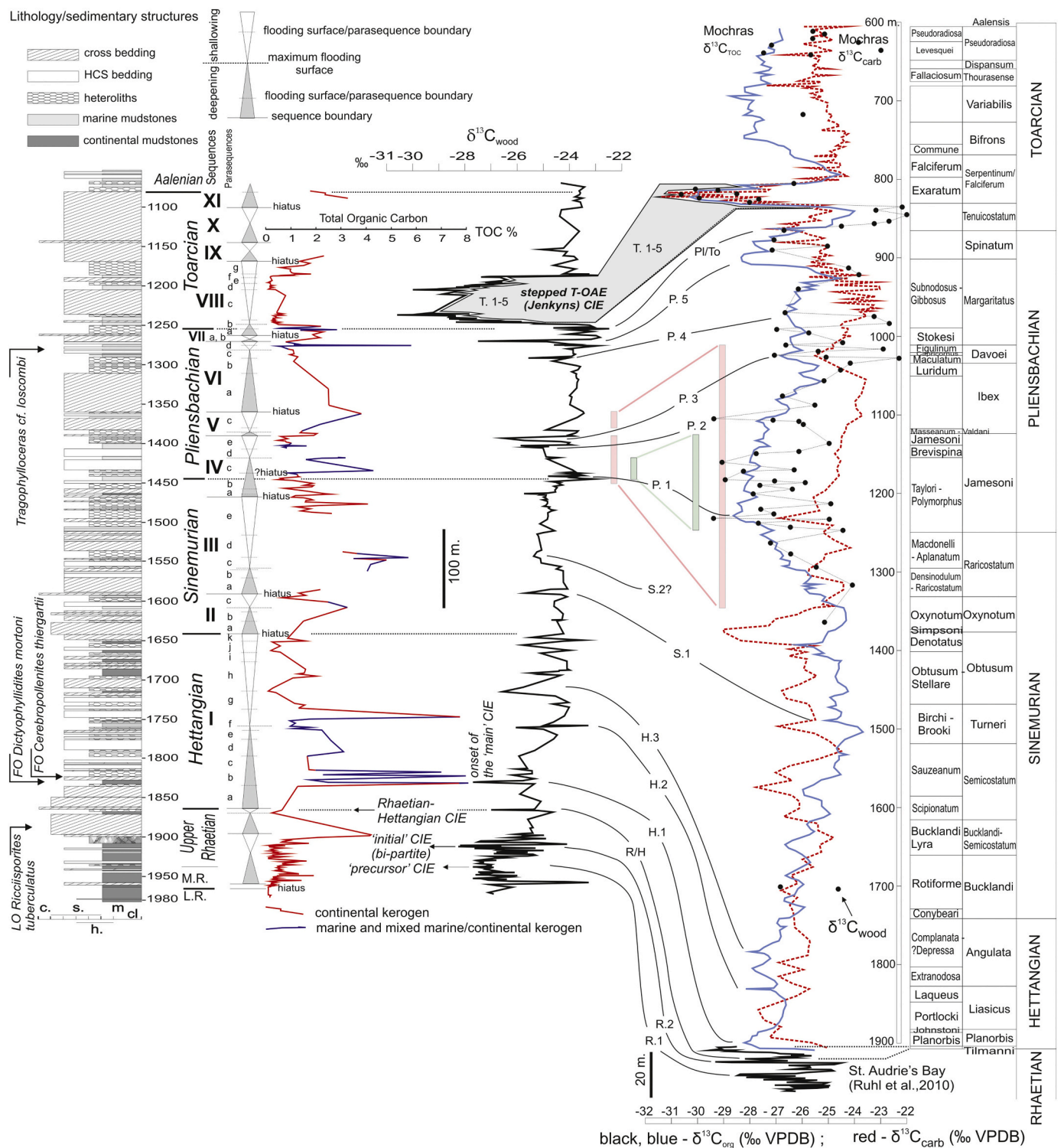
Fig. 2. Stratigraphic correlation between Kaszewy ( \delta^{13}\text{C}_{\text{wood}} - black) and Mochras borehole (blue - \delta^{13}\text{C}_{\text{TOC}} , dashed red - \delta^{13}\text{C}_{\text{carbonate}} and black dots - \delta^{13}\text{C}_{\text{wood}} ), using carbon isotope chemostratigraphy, sequence stratigraphy and biostratigraphical proxies. Reference C isotope curves of the profile Mochras (biostratigraphically calibrated) are based on Storm et al., 2020 ( \delta^{13}\text{C}_{\text{TOC}} , \delta^{13}\text{C}_{\text{wood}} ) and Katz et al., 2005 ( \delta^{13}\text{C}_{\text{carbonate}} ). For the Rhaetian section, the reference curve is based on Ruhl et al. (2010) (black). TOC content in Kaszewy is shown - marine (blue line) and continental (red line). Note two options of chemostratigraphic correlation of the upper Sinemurian - lower Pliensbachian transition. The first option (green bars) implies condensation and incomplete \delta^{13}\text{C}_{\text{wood}} dataset in Kaszewy in the lowermost Pliensbachian, while the second correlation (pink bars) implies strong erosion at the sequence boundaries V and VI, resulting in absence of most of the lower Pliensbachian and atypical (for Polish basin) sedimentary development of both upper Sinemurian and lower Pliensbachian. Considering the above reasons, \delta^{13}\text{C}_{\text{wood}} correlation and correlations with other profiles (Fig. 3), the first option was adopted as more likely, despite more similar general isotope trends when adopting the second option. (For interpretation of the references to colour in this figure legend, the reader is referred to the web version of this article.)
