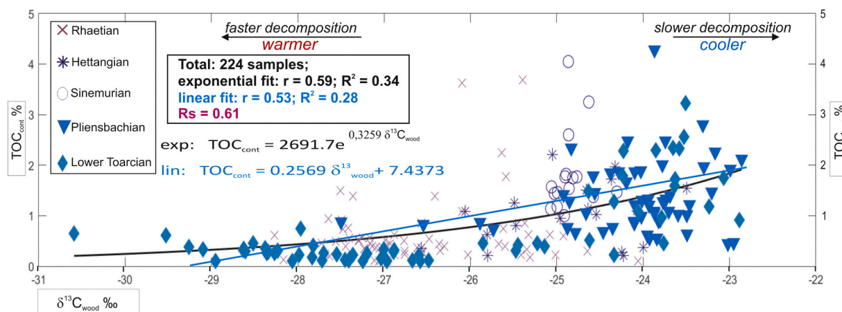
Fig. 5. Plot of \delta^{13}\text{C}_{\text{wood}}/\text{TOC}_{\text{cont}} showing statistically significant positive correlation (Pearson) between the two variables in 224 samples, both for linear (lin) and exponential (exp) fit: r = 0.59 for exponential fit; r = 0.53 for linear fit. The p -value is < 0.00001 . The result is statistically significant at p < .05 . For the Rhaetian (66 samples) r = 0.16 ; for the Lower Jurassic (159 samples) r = 0.57 ; Spearman's Rank Correlation Coefficient (in 224 samples): R_s = 0.61 , p \text{ val} = 6.44 \times 10^{-24} ; the result is significant the significance threshold 0.001 (see Supplementary 4). The correlation is interpreted as a result of differentiated decomposition of terrestrial organic matter related to climate changes, but also other factors could have influenced the observed relationship.
