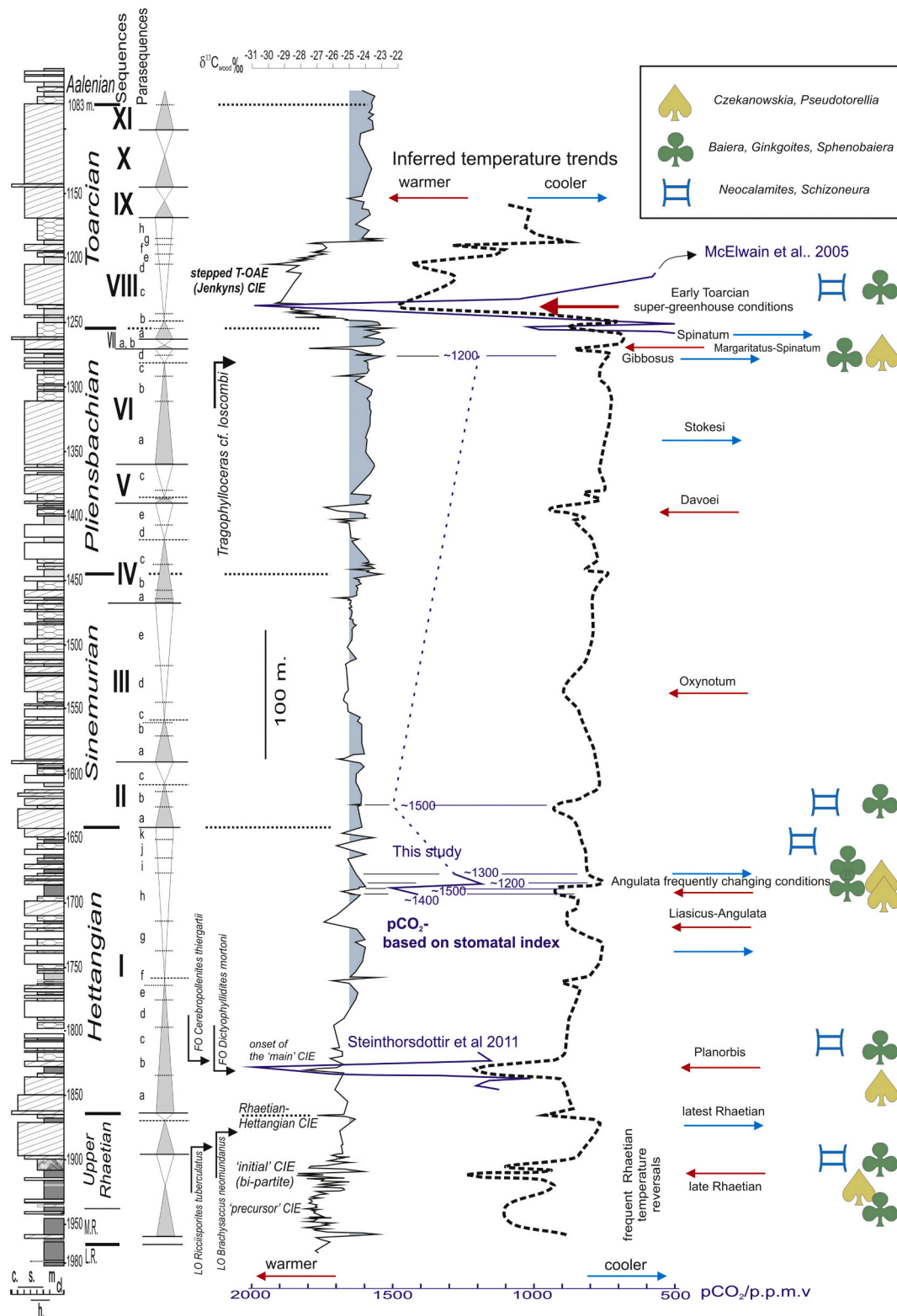
Fig. 7. Inferred temperature trends in Rhaetian and Early Jurassic in the Kazswey profile based on stomatal index and macrofloral data and tentatively on the \delta^{13}\text{C}_{\text{wood}}/\text{TOC}_{\text{cont}} plot (Fig. 5). Macroflora represents three general assemblages: Czekanowskia-Pseudotorellia (relatively drier-cooler conditions), Baiera-Ginkgoites-Sphenobaiera (relatively warmer and more humid) and Neocalamites-Schizoneura (humid). Climatic trends are indicated with their inferred stratigraphic age.
