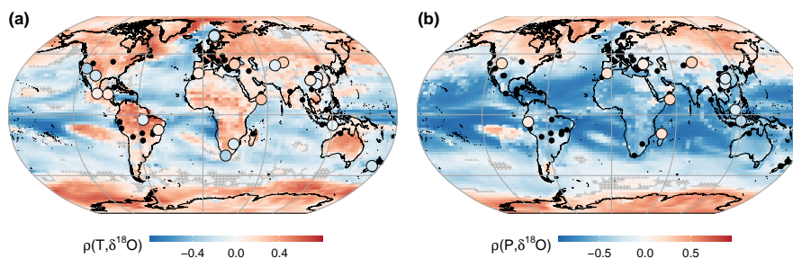
Figure 7. Correlation fields of simulated \delta^{18}\text{O} and the related climate variables surface temperature (a) and precipitation (b) for simulation LM1 ( |c| > 0.2, p < 0.1 ). Colored symbols give the correlation between simulated climate variables and the \delta^{18}\text{O}_{\text{dw.eq}} of the speleothem records. Empty tiles mask insignificant correlations. Black dots show cave locations with insignificant correlations.
