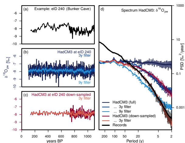
Figure 6. Variability on different time scales through comparison of measured \delta^{18}\text{O}_{\text{dw.eq}} and simulated \delta^{18}\text{O} time series as well as of their spectra. (a-c) Example time series of eID 240 in Bunker cave (Germany) (Fohlmeister et al., 2012). (a) The measured \delta^{18}\text{O}_{\text{dw.eq}} in the speleothem, (b) the iHadCM3 simulated \delta^{18}\text{O}_{pw} at the cave location with two filters (3 and 9 years) and (c) the simulated \delta^{18}\text{O}_{pw} but down-sampled to the same temporal resolution as in (a) with 3 year filter. (d) Power spectral density (PSD) of mean spectra of simulated \delta^{18}\text{O}_{pw} at the cave site in yearly resolution (blue), down-sampled to the caves resolution (red) and mean spectrum of the \delta^{18}\text{O}_{\text{dw.eq}} of the records (black), including the karst-filters as shown in (a-c). The spectra are area-weighted and averaged over the three simulations (LM1, LM2 and LM3). The colors for the example eID in (a-c) correspond to the colors of the mean spectra over all entities in (d).
