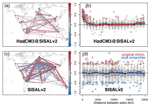
Figure 8. Network spanned by the 5% strongest absolute correlations of simulated iHadCM3 \delta^{18}\text{O} at the SISAL cave sites (a, down-sampled). All model-based between-site-correlations are shown in the distance-binned boxplot (b). Network visualizations (c) and distance-binned boxplot (d) of the cross-correlations between SISAL site \delta^{18}\text{O}_{\text{speleo}} for the original age models. The color values indicate the 5% strongest correlations in network and boxplot. The LOESS smoother (span = 0.2) in the boxplots indicate the correlation for the original chronology (red) as well as the absolute highest correlation through selection of age-models (blue).
