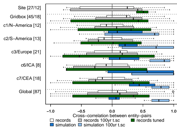
Figure 9. Cross-correlation on site, gridbox, clusters and global scale for speleothem records and the locally interpolated model output for \delta^{18}\text{O} . 12 (18) sites (gridboxes) contain more than one speleothem entity with a total of 27 (45). At each aggregation level the correlations between all entities is shown for \delta^{18}\text{O}_{\text{speleo}} (white bars), and the down-sampled model output \delta^{18}\text{O} at cave locations (blue bars). Different temporal scales (original resolution and 100yr-timescale (t.sc)) are compared as well as the age-model ensemble that gives the highest absolute correlation (dark green bars). Clusters are indicated with the number of speleothem entities in brackets, where c4, c5, c8, and c9 are not included because they contain too few entities. c6/ICA is the India and Central Asia cluster, c7/CEA is the China and Eastern Asia cluster.
