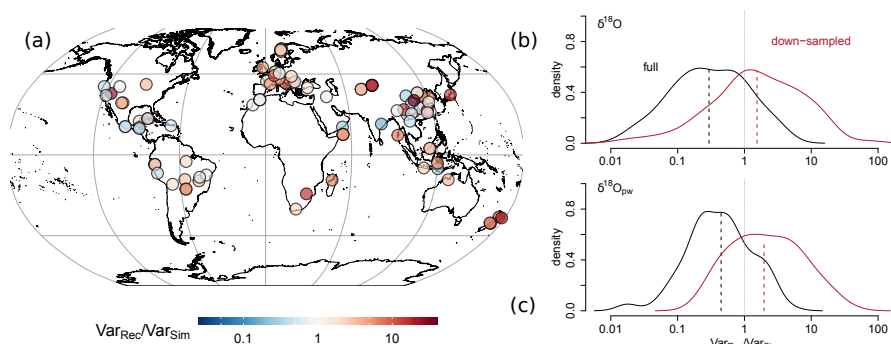
Figure 5. (a) Spatial visualization of the site-based dimensionless variance ratio V_{Rec}/V_{Sim} based on LM1. Aggregated density plots of the variance ratio of \delta^{18}O (b) and precipitation-weighted \delta^{18}O (c) for the raw records ('full', black lines) and where the simulation has been down-sampled to the record resolution ('down-sampled', red lines) illustrate the variance loss due to temporal averaging in the archive (uses LM1-3).
