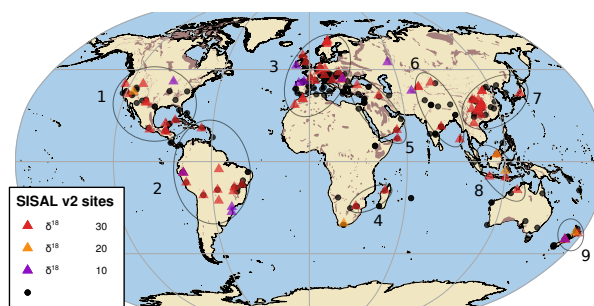
Figure 2. Site locations of the SISAL database on a global karst map (brown shadings Williams and Ford, 2006). The sites with entities that pass the prerequisites for our analysis are marked in colored triangles. These entities cover at least a period of 600yr within the last millennium and have a minimum of 30 (red), 20 (orange), or 10 (purple) \delta^{18}\text{O} measurements and two dating points in this period. All other sites in the SISAL database v.2. are marked with a black dot. The nine clusters used in the analysis here are North America (c1, 12 entities), South America (c2, 13 entities), Europe with North Africa (c3, 21 entities), Southern Africa (c4, 2 entities - too few for systematic analysis), Middle East (c5, 6 entities), India and Central Asia (c6, 8 entities), East Asia (c7, 18 entities), South East Asia (c8, 4 entities), and New Zealand (c9, 3 entities).
