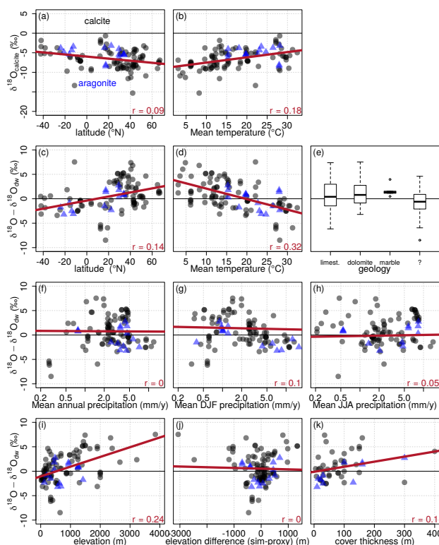
Figure 4. Systematic comparison of climate variables and cave parameters on \delta^{18}\text{O}_{\text{dw.eq}} and the offset \Delta\delta^{18}\text{O} to the simulation. Shown are the absolute values of \delta^{18}\text{O}_{\text{dw.eq}} against: (a) site latitude, and (b) simulated local annual mean temperature, and the model-data difference against (c) latitude, (d) simulated mean annual temperature, (e) geology surrounding the cave ('?' means unknown geology), (f) mean annual (g) DJF and (h) JJA precipitation amount as well as (i) cave elevation, (j) the elevation difference between the model grid and actual cave, and (k) the overall cover thickness above cave. Symbols denote calcite (black circles) or aragonite (blue triangles) specimens. An unweighted linear regression (red line) is added for illustration, but without consideration of significance.
