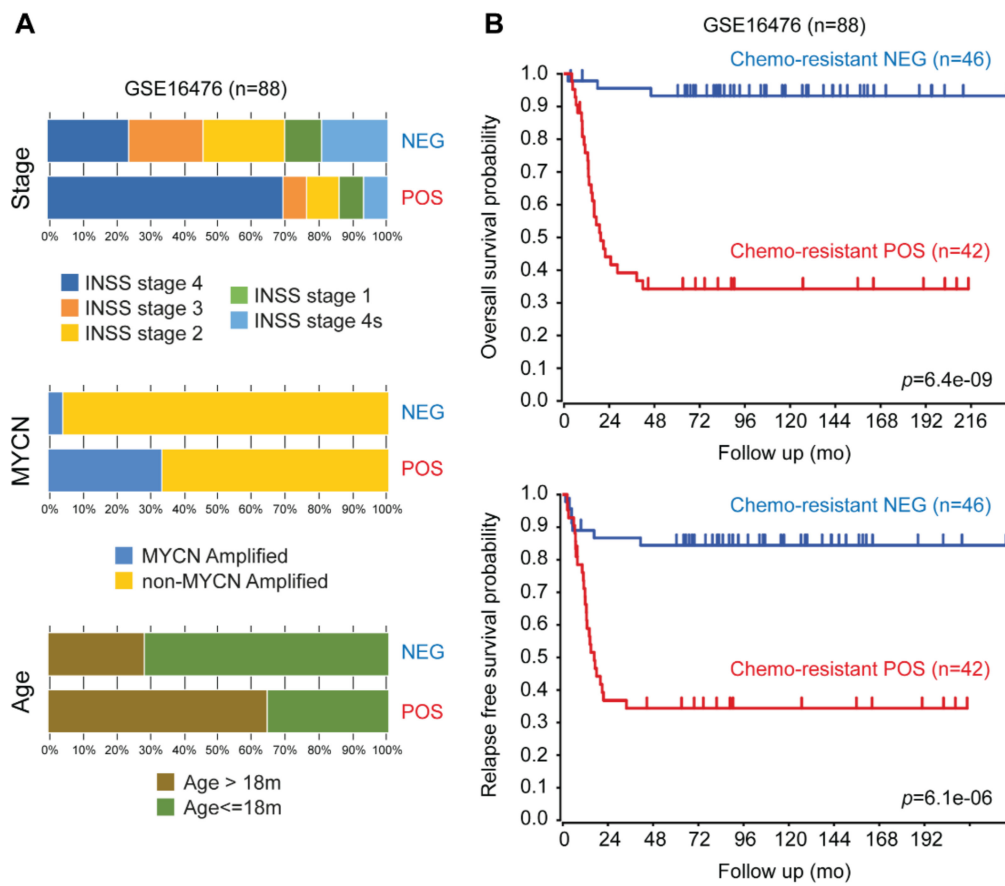
Figure 5. Chemo-resistant POS groups have worse overall survival probabilities as compared with chemo-resistant NEG and worse relapse-free survival probabilities over time. (A) The stacked bar plot shows the phenotypic features of samples in GSE16476 stratified by k-means clusters. For this dataset we report the International Neuroblastoma Staging System (INSS) Stage, MYCN amplification status, and age at diagnosis grouped by the 18 months cutoff. (B) Kaplan–Meier curves calculated by the log-rank test showing the overall and the relapse-free survival probabilities for GSE16476. p -values were calculated with log-rank test. All the analyses were performed on the R2 web platform ( http://r2.amc.nl ).
