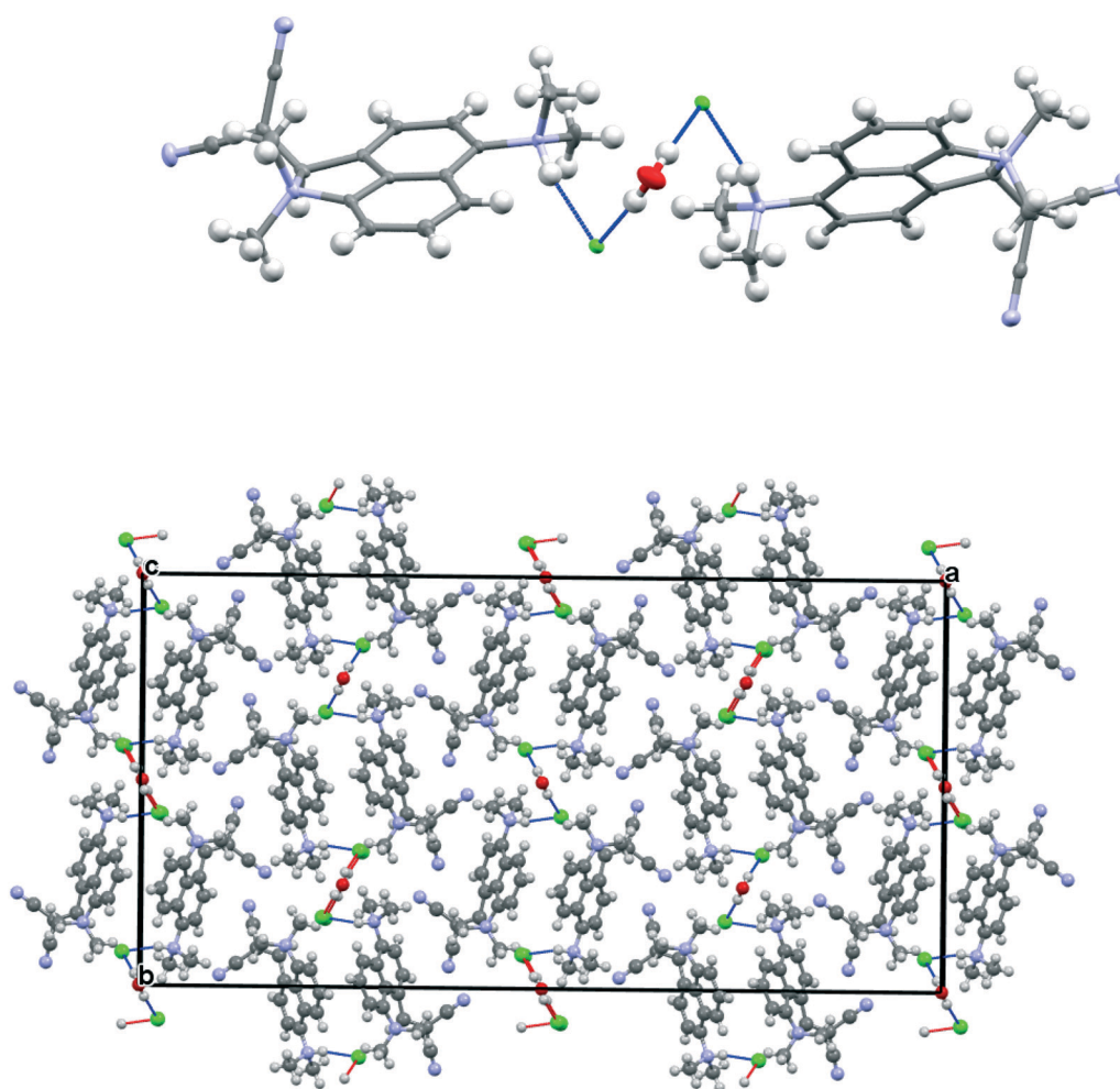
Fig. 4 Crystal packing for 13 ·Cl - ·0.5H 2 O at 100 K viewed down the c axis: a pair of chloride anions bridged by a water molecule each form a hydrogen bond to the N-H of the dimethylammonium group of cation 13 (above) and the full crystal packing arrangement (below).
