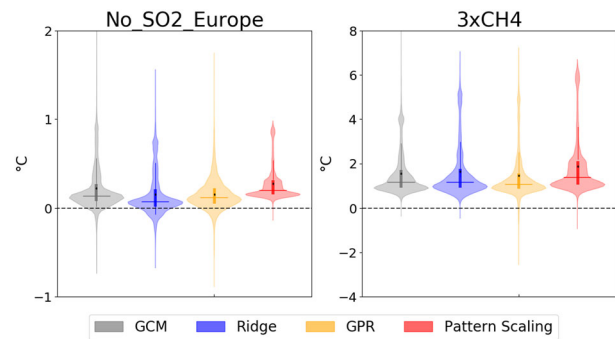
Fig. 2 Distribution of predicted grid-point scale surface temperature responses in °C for all methods for one short-lived forcing, No_SO 2 Europe, and one long-lived forcing, 3xCH 4 . The central vertical boxes indicate the interquartile range shown on a standard box plot, the horizontal line shows the median and the black point shows the mean. The horizontal width shows the distribution of temperature values overall grid points, i.e. the wider regions highlight that more grid points have this value of predicted temperature response. Note the different vertical scales.
